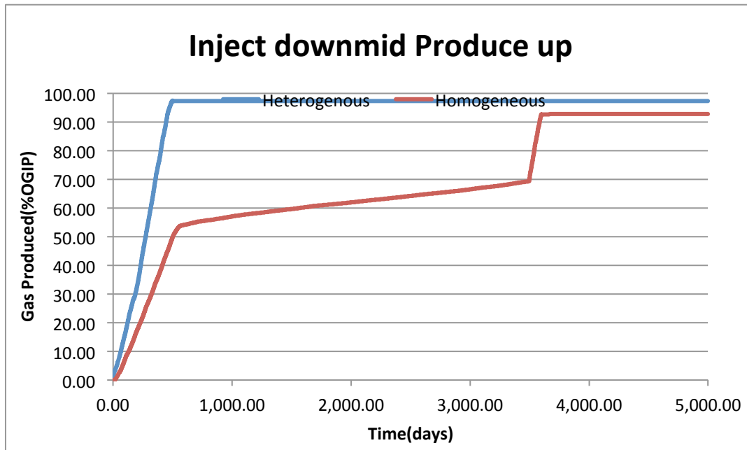
Figure 7.2.c.3: Gas production for homogeneous and heterogeneous ‘inject downmid produce up’ reservoir
