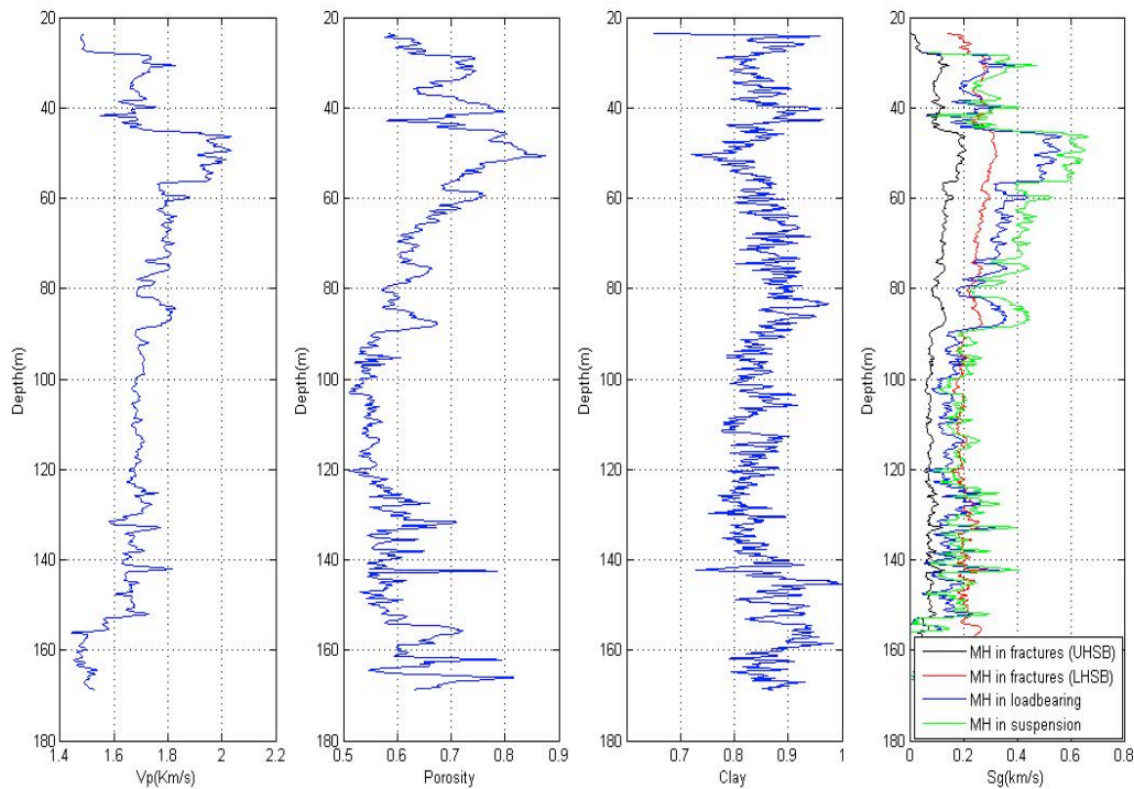
Figure 19: Results from Krishna-Godavari Basin offshore East Cost India. From left to Right: (A) compressional wave velocity (Km/s) with respect to depth (m); (B) Porosity with respect to depth (m); (C) Clay content with respect to depth (D) Hydrate saturation with respect to depth (m) using different rock physics models: (green) soft rock model adjusted for suspension state. (Blue) soft rock model adjusted for loadbearing state.
