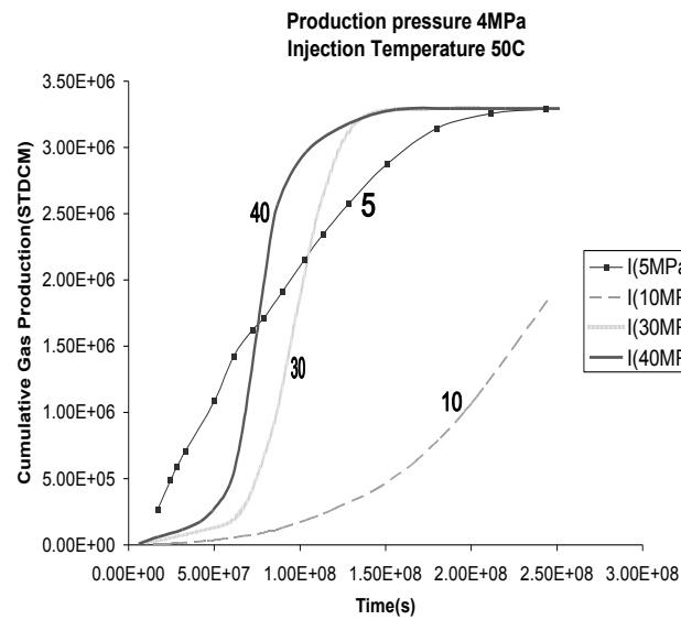
Figure 7.2.a.5: Cumulative gas production with varying injection pressure and 4MPa of production pressure and 50°C of injection temperature.
