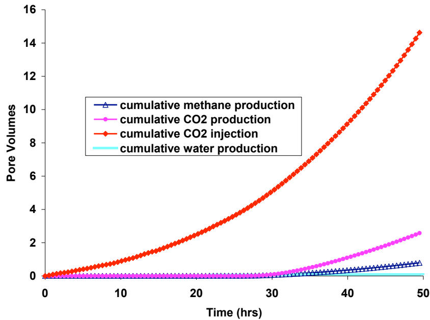
Figure 7.2.d.4: Cumulative methane production, \text{CO}_2 production and \text{CO}_2 injection
