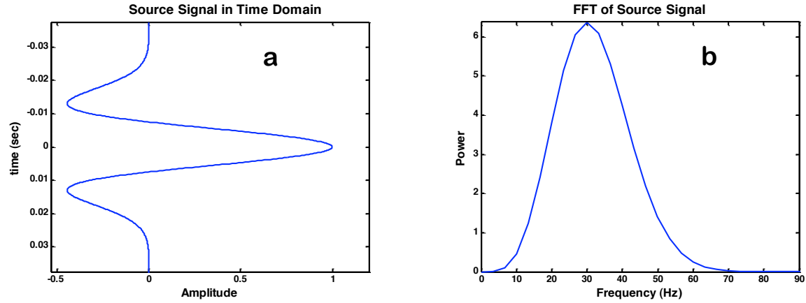
Figure 9. A sample Ricker wavelet, f_{\text{peak}}=30 Hz; (a) In time domain; (b) Power spectrum in frequency domain
