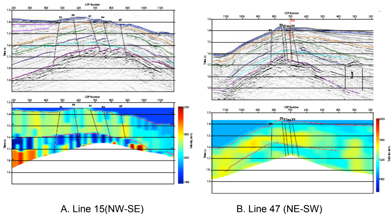
Figure 2. Multichannel Seismic. Top A and B: The interpreted section; light blue color represents BSR. Bottom A and B. The velocity model from the conventional semblance analysis method for stacking velocity estimation; blue is slower velocity and red is faster velocity. Water bottom and BSR are highlighted on the velocity model. A drop in interval velocity is observed below the BSR (free gas?) and several high velocity patches (hydrates?) are observed above the BSR.
