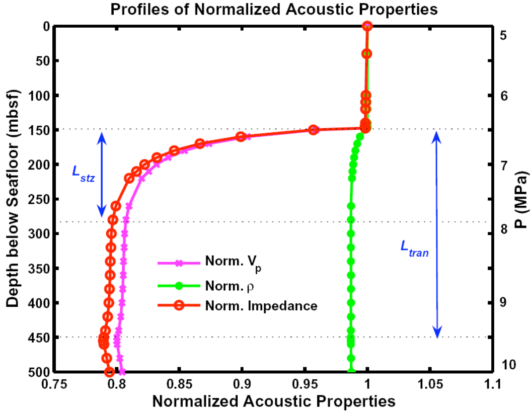
Figure 6. Profiles of normalized acoustic properties in an example \text{CH}_4\text{-C}_3\text{H}_8\text{-H}_2\text{O} System. Conditions are the same as Figure 3. Impedance Z = \rho V_p . Data are normalized to those at seafloor.
