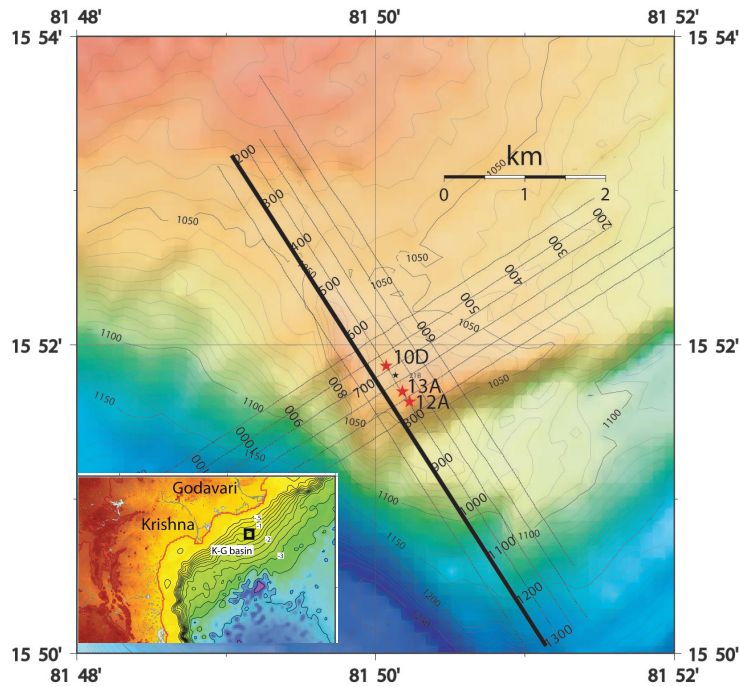
Figure 6. Bathymetry map of the study area. Location with respect to the Indian east-coast is shown in inset. Seismic line released for this study by Indian Govt. is shown in bold. Other available survey lines for future release are shown in grey. Wells 10D, 13A, and 12A, were logged/cored during NGHP-01 expedition. Data from these wells are in public domain.
