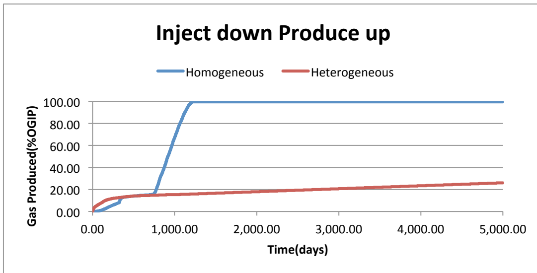
Figure 7.2.c.4: Gas production for homogeneous and heterogeneous ‘inject down produce up’ reservoir
