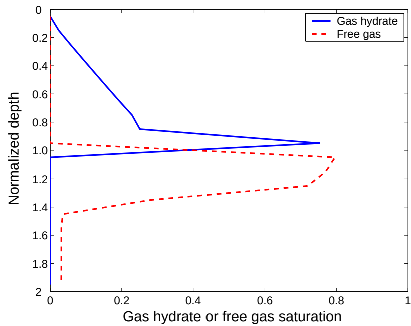
Figure 10.7: Gas hydrate and free gas saturation profiles at the critical-state for N_{sc} = 1000 . A deep connected free gas column forms beneath the GHSZ and is trapped by the high saturation hydrate layer.
