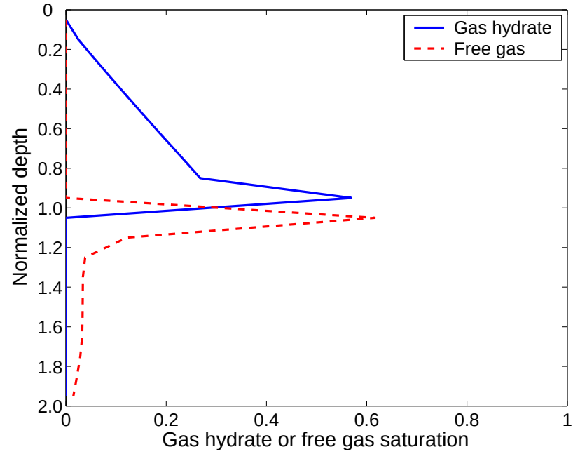
Figure 10.5: Gas hydrate and free gas saturation profiles at time \tilde{t} = 1 for N_{sc} = 1000 .
