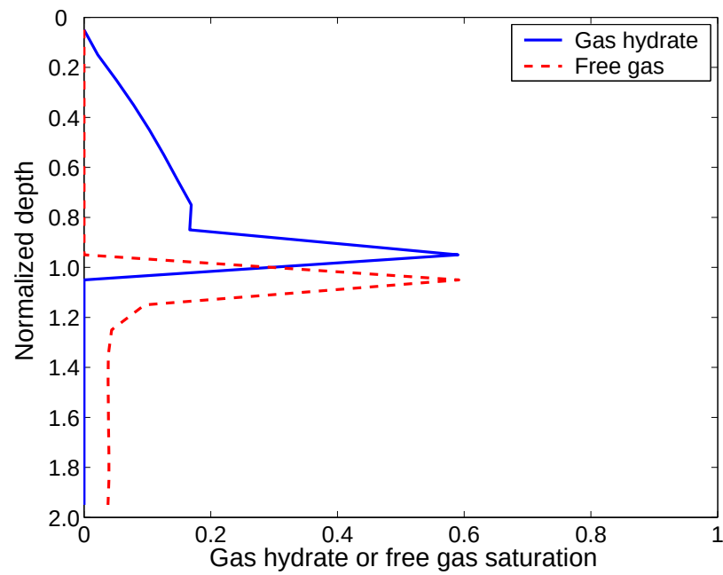
Figure 10.10: Gas hydrate and free gas saturation profiles at the critical-state for N_{sc} = 10 ( \tilde{t} \sim 1.5 ). Compared to the thick gas column in Figure 10.7, only a relatively thin free gas column forms beneath the GHSZ in this case before gas pressure becomes equal to the overburden.
