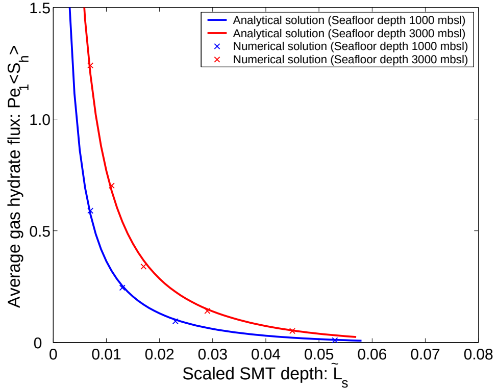
Figure 8.8: Relationship between average gas hydrate flux ( Pe_1\langle S_h \rangle ) and scaled SMT depth ( \tilde{L}_s ) for different seafloor depths. Curves representing analytical solutions are also compared with steady state numerical simulations of Bhatnagar et al. (2008). Shallow SMT depths indicate higher methane flux from deeper sources causing higher average gas hydrate flux (and saturations) through the GHSZ.
