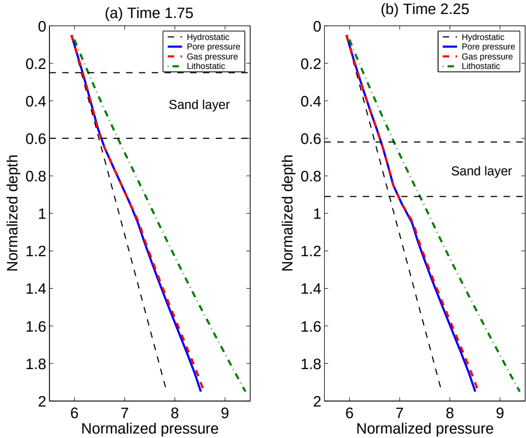
Figure 10.18: Pressure evolution for the case of a sand layer (high permeability) deposited in low permeability sediments uniformly across the lateral section. Sand layer is deposited from time \tilde{t} = 1.0 to 1.5. (a) Pore pressure, gas pressure and lithostatic stress profiles along depth at time \tilde{t} = 1.75 . The dotted interval represents the sand layer and is characterized by pore pressure gradient that is close to the hydrostatic gradient. (b) At a later time, \tilde{t} = 2.25 , the sand layer moves deeper and shrinks in thickness due to compaction.
