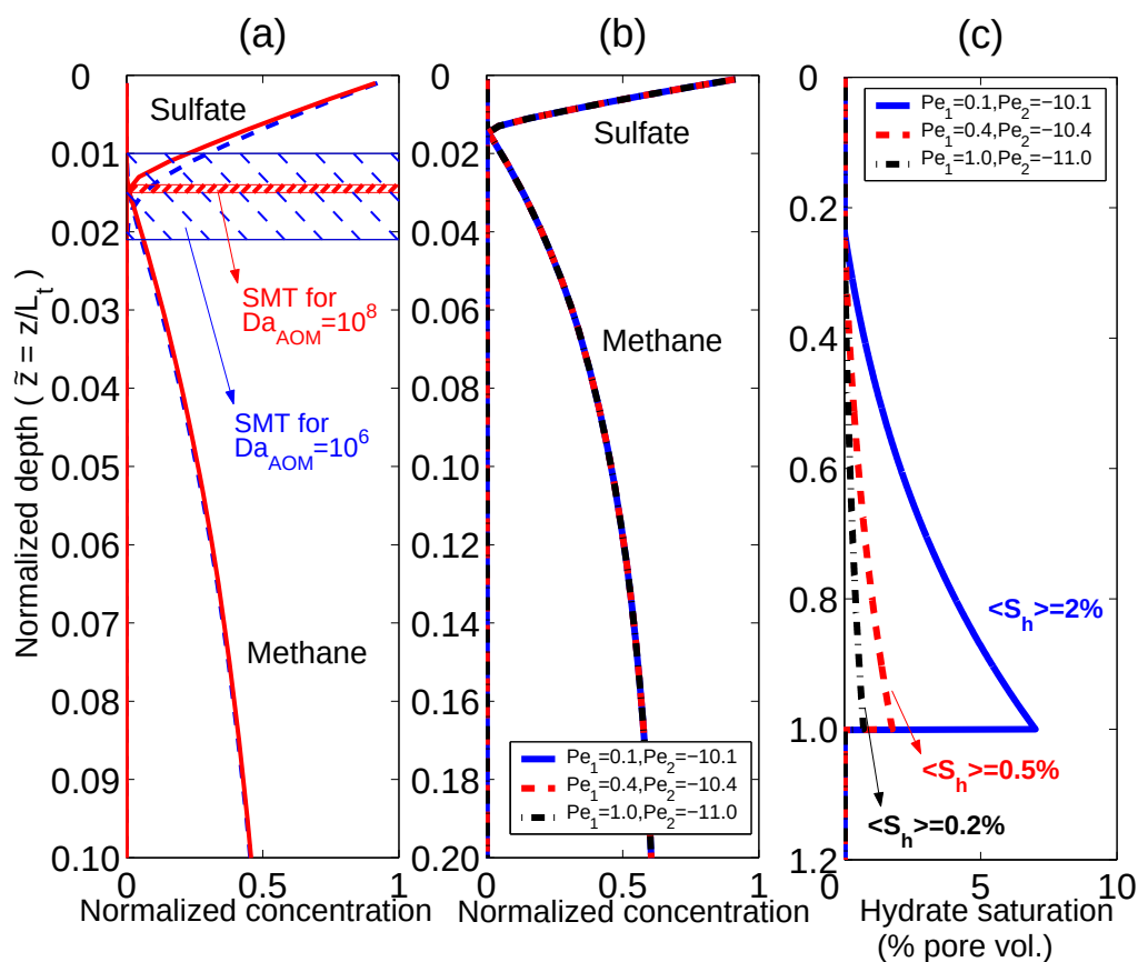
Figure 7.2: Effect of Damkohler number ( Da_{AOM} ) and Peclet numbers ( Pe_1, Pe_2 ) on steady state profiles. Pe_1 + Pe_2 = -10 for all simulations (Note different y-axis scale for each plot). (a) Sulfate and methane profiles for Da_{AOM} = 10^8 (solid curves) and Da_{AOM} = 10^6 (dashed curves). The hatched regions compare the thickness of the SMT zone for the two cases. (b) Simulations for different sets of Pe_1 and Pe_2 , but with Pe_1 + Pe_2 = -10 . Overlap of methane and sulfate profiles shows that the sum Pe_1 + Pe_2 controls the concentrations. (c) Gas hydrate saturation profiles do not depend only on Pe_1 + Pe_2 , because different Pe_1 causes distinct residence times of gas hydrate within the GHSZ.
