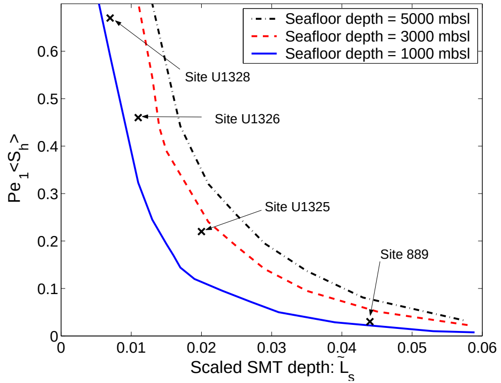
Figure 7.4: Relationship between Pe_1\langle S_h \rangle and scaled SMT depth ( \tilde{L}_s = L_s/L_t ) for several seafloor depths. Points corresponding to different Cascadia Margin sites are plotted to show how AGHS can be estimated from \tilde{L}_s using this plot (Table 7.1).
