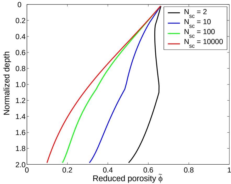
Figure 9.4: Effect of the parameter N_{sc} on steady-state reduced porosity profiles. At relatively high values of N_{sc} , pore pressure remains close to hydrostatic, causing equilibrium compaction and maximum porosity loss. As N_{sc} is reduced, pore pressure increases from hydrostatic values, resulting in lower effective stresses, lesser compaction and significantly higher porosities.
