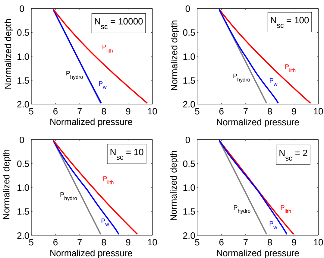
Figure 9.2: Effect of the sedimentation-compaction parameter N_{sc} on steady state pore pressure profiles. Lower values of N_{sc} imply higher sedimentation rates and/or lower permeabilities resulting in pore pressures higher than hydrostatic. Each pore pressure curve is bounded by the hydrostatic pressure profile as the lower limit and the lithostatic stress profile as the upper limit. At relatively higher values of N_{sc} pore pressure is almost hydrostatic, whereas relatively lower values of N_{sc} lead to almost lithostatic pore pressures.
