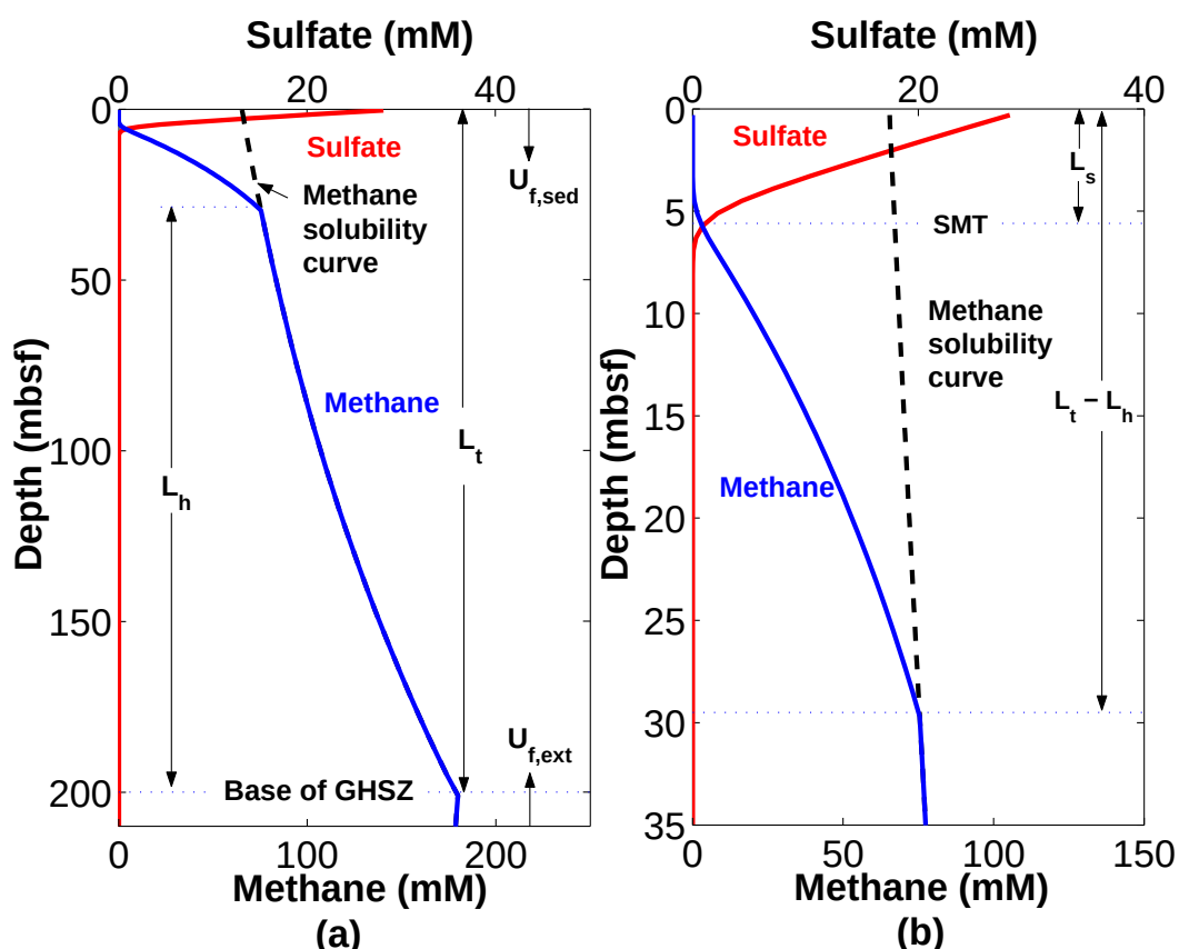
Figure 8.1: (A) Schematic representation of a gas hydrate system showing pore water sulfate and methane concentrations, which go to zero at some shallow depth because of anaerobic oxidation of methane (AOM). Also shown are methane solubility in water, the two fluid fluxes ( U_{f, sed} and U_{f, ext} ), and depth to the base of the gas hydrate stability zone ( L_t ). (B) Close-up of the sulfate-methane transition (SMT) showing overlap of sulfate and methane profiles, its depth below the seafloor ( L_s ), and the depth to the top of the gas hydrate layer ( L_h ).
