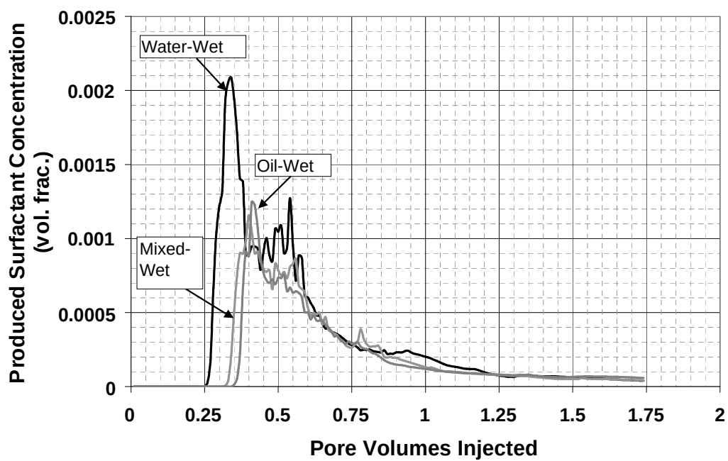
Fig. 4.3-10. Produced Surf. Conc. for Constant Wettability Simulations
