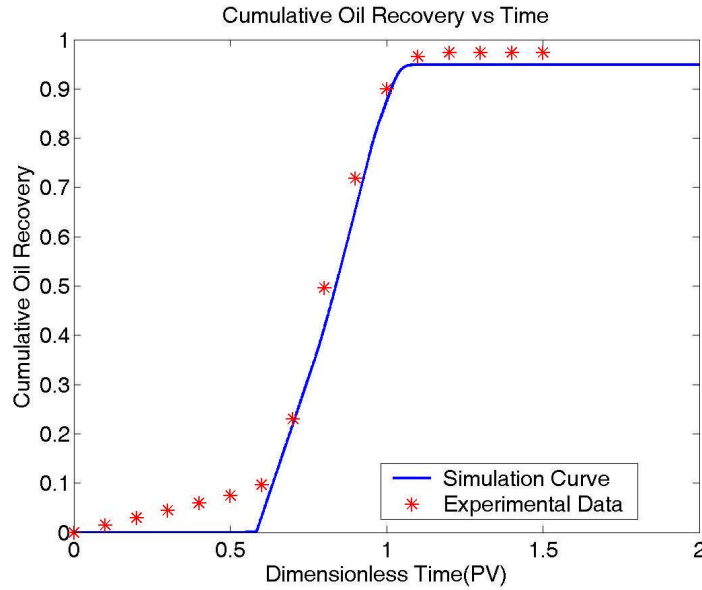
Figure 2.4-11 Comparison between simulation and experiments for silica pack
