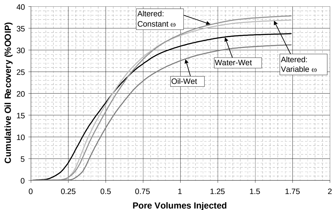
Fig. 4.3-14. Cumulative Oil Recovery for Wettability Alteration Simulations
