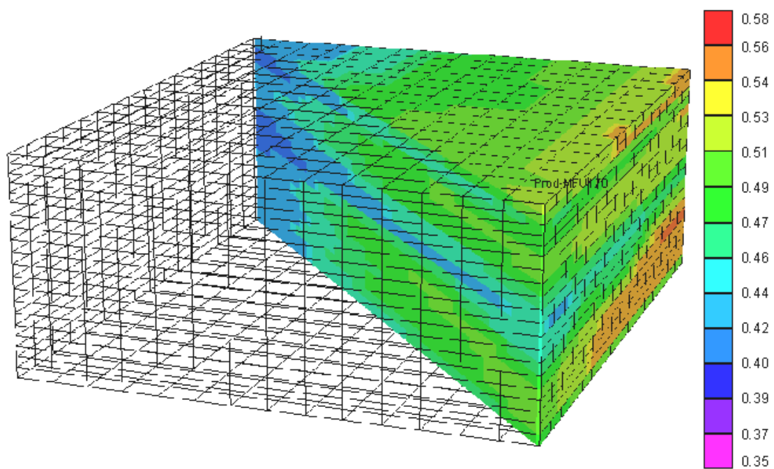
Fig. 4.3-2. Simulation Model Initial Oil Saturation
