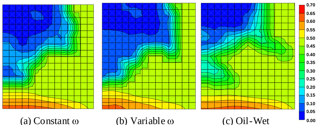
Fig. 4.3-22. Comparison of Oil Saturation at 0.85 PV in Layer 4
