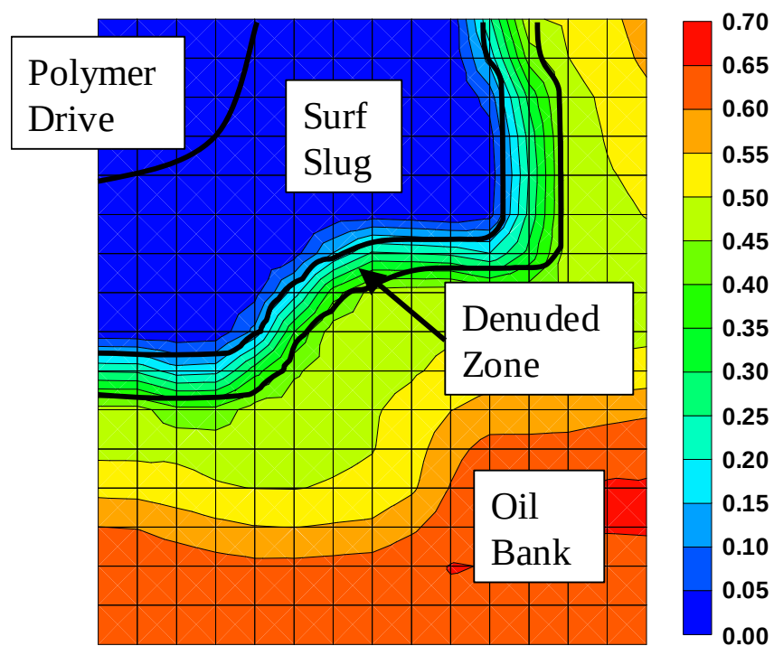
Fig. 4.3-17. Example Oil Saturation Profile
