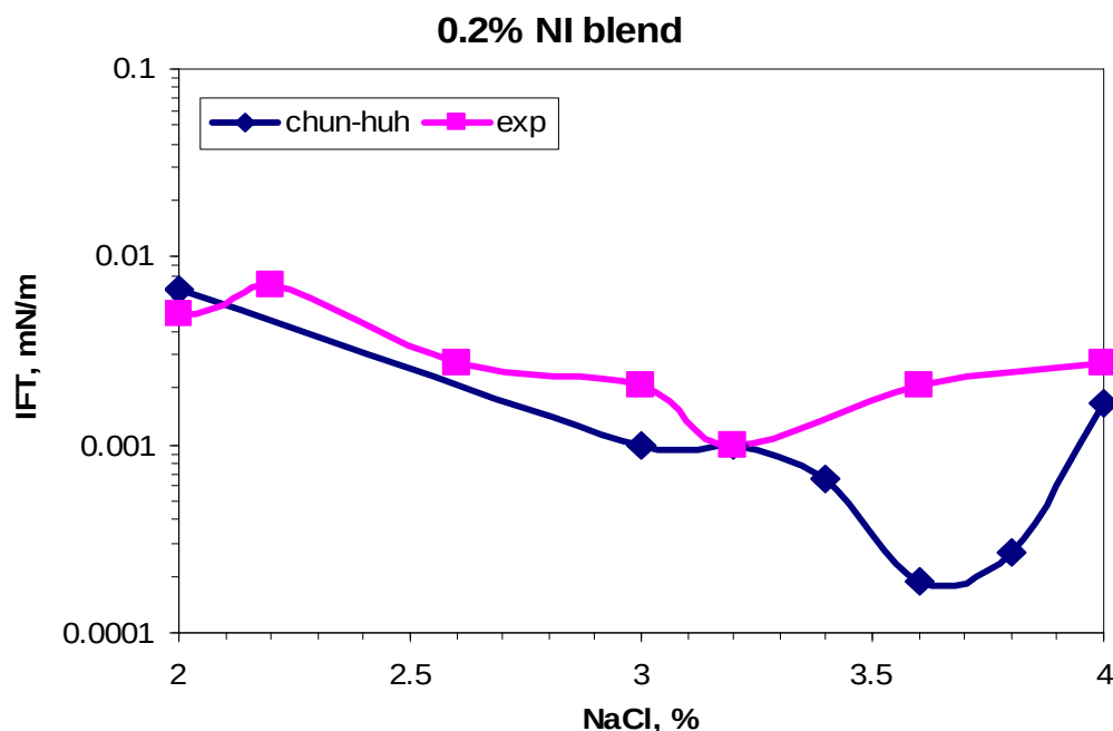
Figure 2.2-22 Comparison of IFT measured by spinning drop measurements using standard procedure and that estimated by Chun-Huh correlation of 0.2% NI blend/1% \text{Na}_2\text{CO}_3/\text{NaCl} . c=0.3 .
