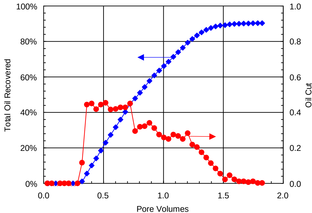
Figure 1.4-1 Oil recovery during Berea core flood B-1.
