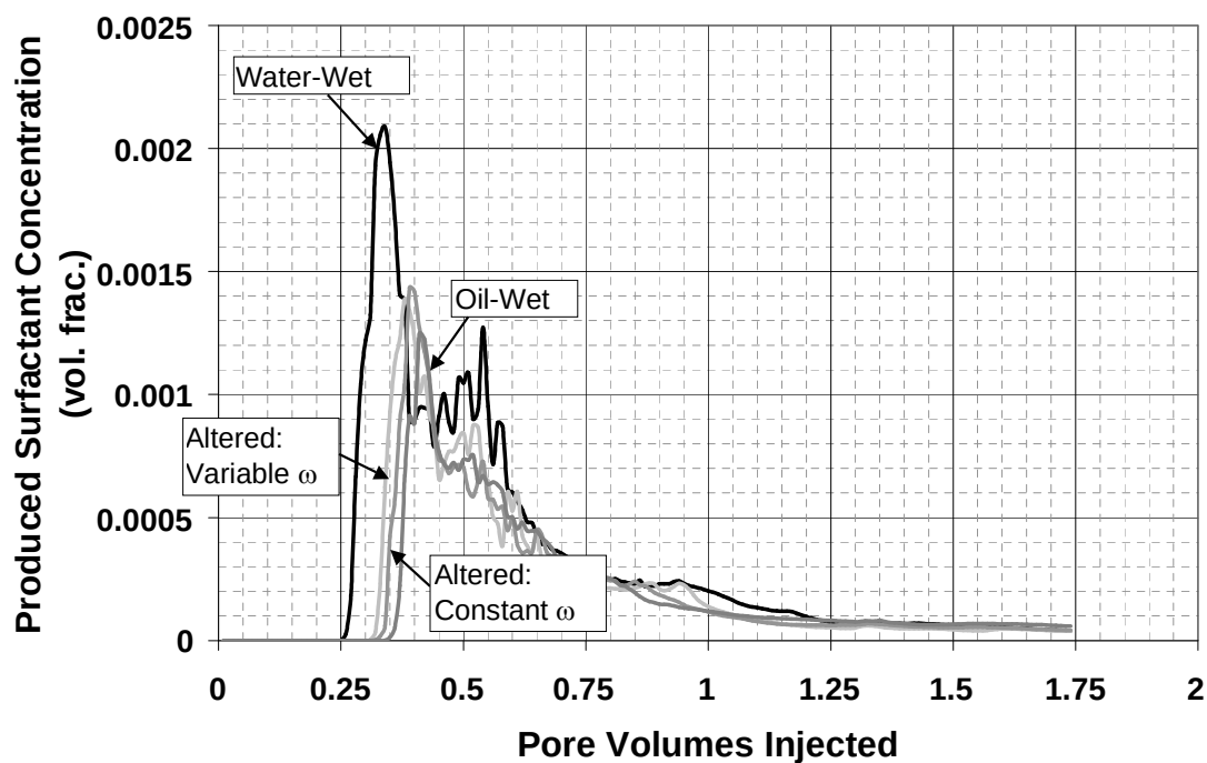
Fig. 4.3-16. Produced Surf. Conc. for Wettability Alteration Simulations
