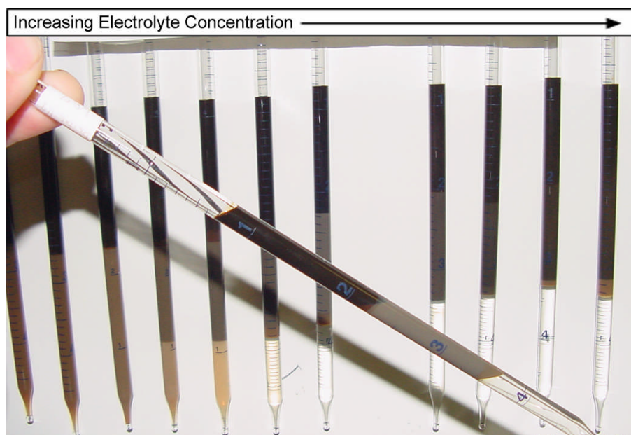
Figure 1.2-9 Qualitative observations of phase behavior, interface fluidity and viscosity by tilting pipettes.
