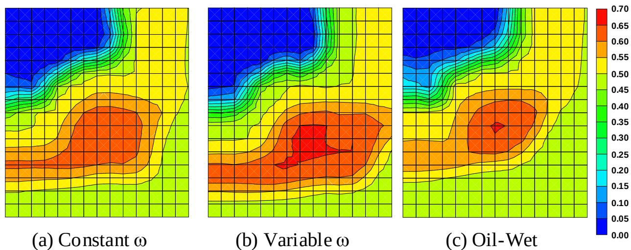
Fig. 4.3-18. Comparison of Oil Saturation at 0.2 PV in Layer 4
