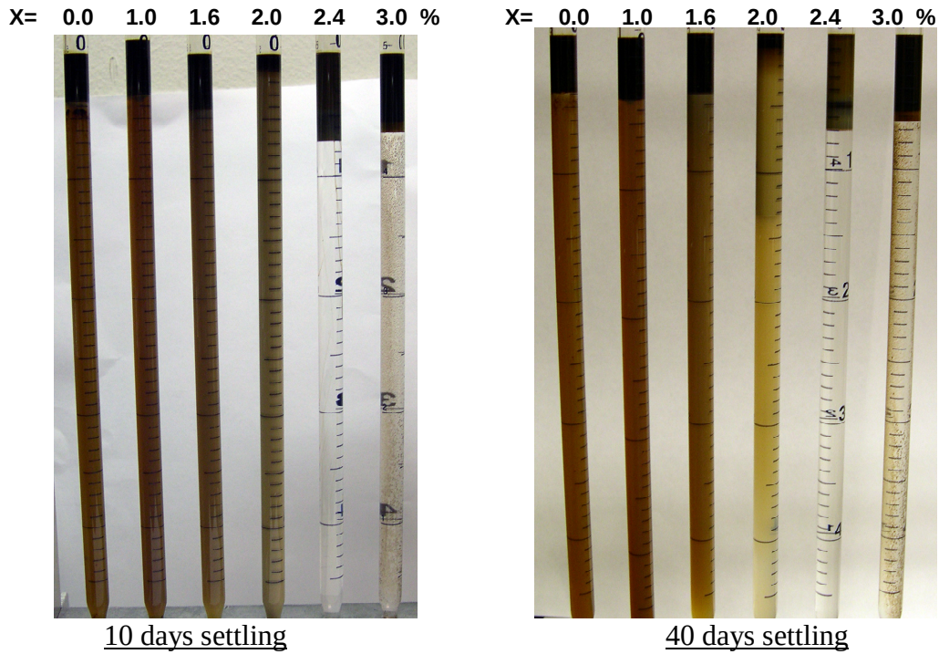
Figure 2.5-2 Phase behavior of White Castle with 0.2% NI / 1% \text{Na}_2\text{CO}_3 / x% NaCl, WOR=9:1 , 24 hours mixing at different settling time.
