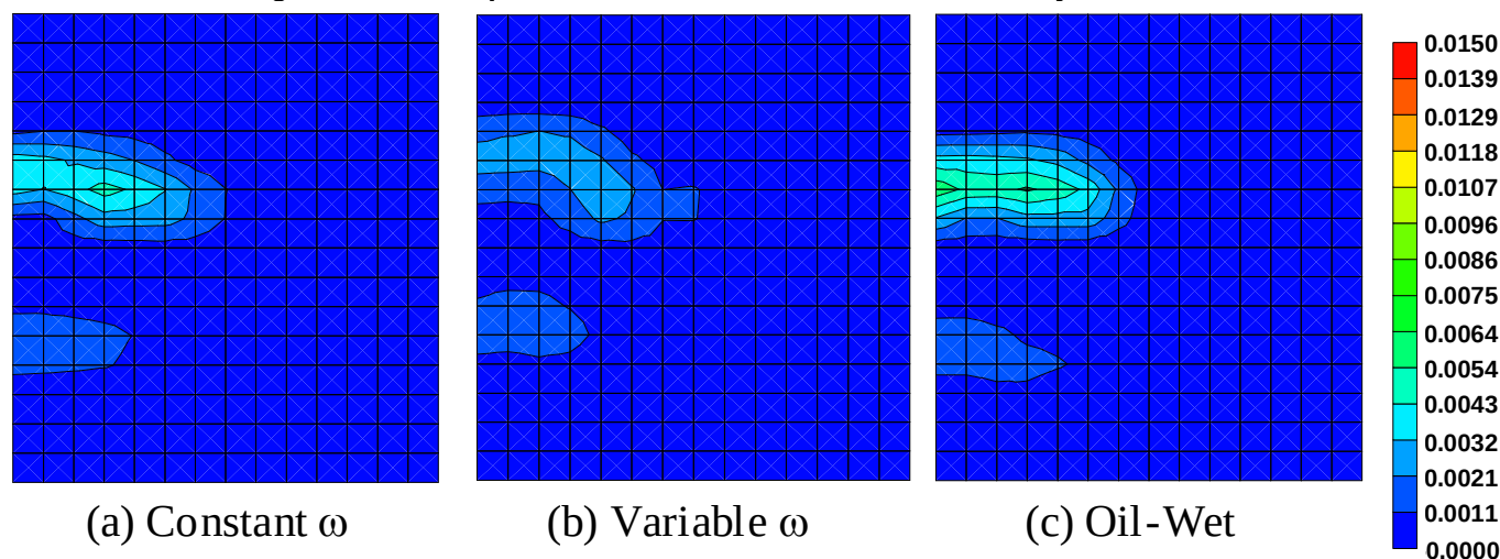
Fig. 4.3-23. Comparison of Surf. Conc. (vol frac) at 0.85 PV in Layer
