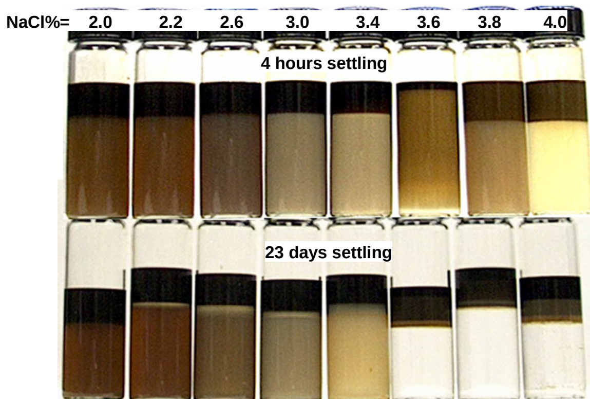
Figure 2.2-9 Comparison of phase appearance of 0.2% NI / 1% \text{Na}_2\text{CO}_3 / x % NaCl at different time
