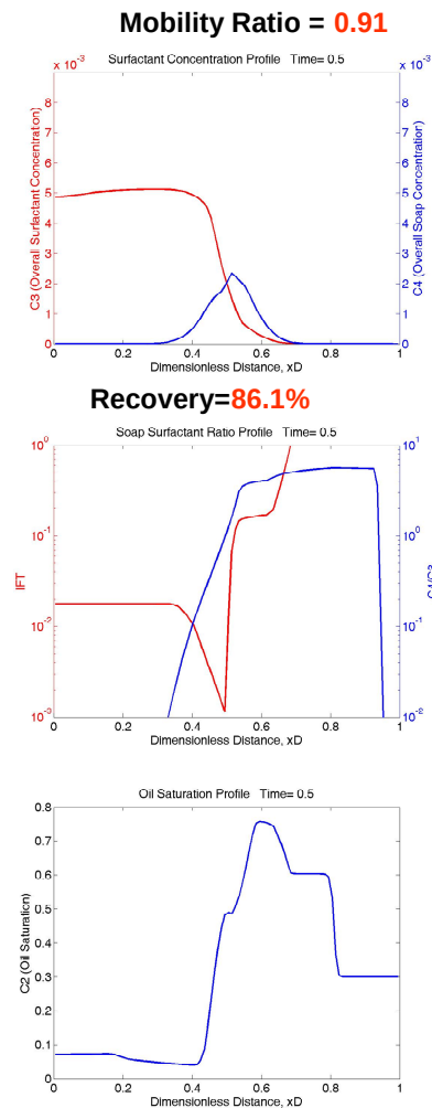
Figure 2.3-5 Comparison of profiles between varied injecting solution viscosities
