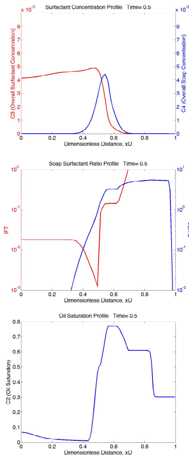
Figure 2.3-3 Comparison of profiles between wide low IFT region and narrow low IFT region
