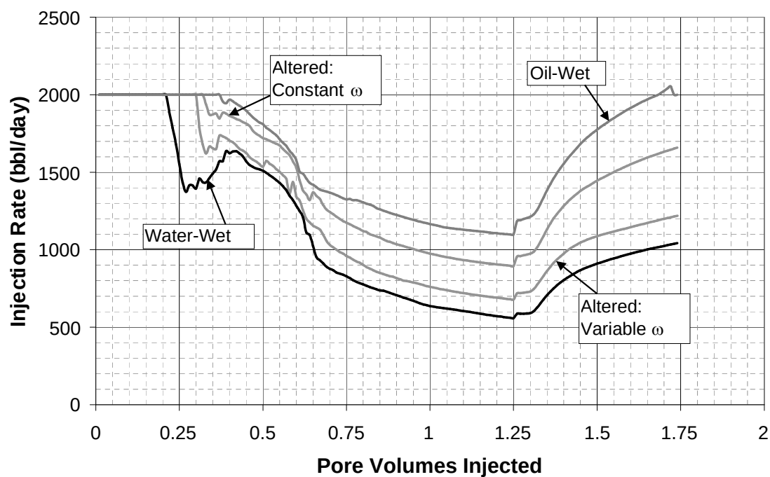
Fig. 4.3-13. Injection Rates for Wettability Alteration Simulations
