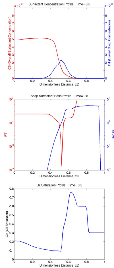
Figure 2.3-3 Comparison of profiles between wide low IFT region and narrow low IFT region
