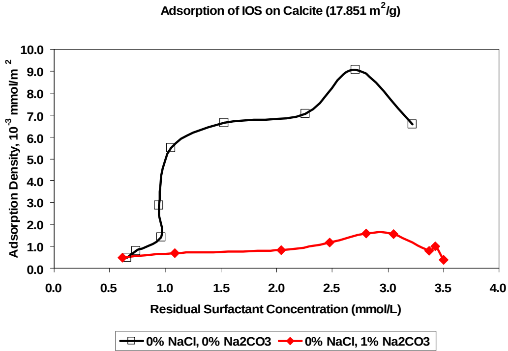
Figure 2.1-5 Adsorption of IOS on calcite powder
