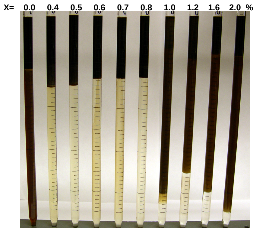
Figure 2.5-1 Phase behavior of White Castle with 0.2% NI / 1% \text{Na}_2\text{CO}_3 / x% NaCl, WOR=3:1 , 24 hours mixing, 40 days settling
