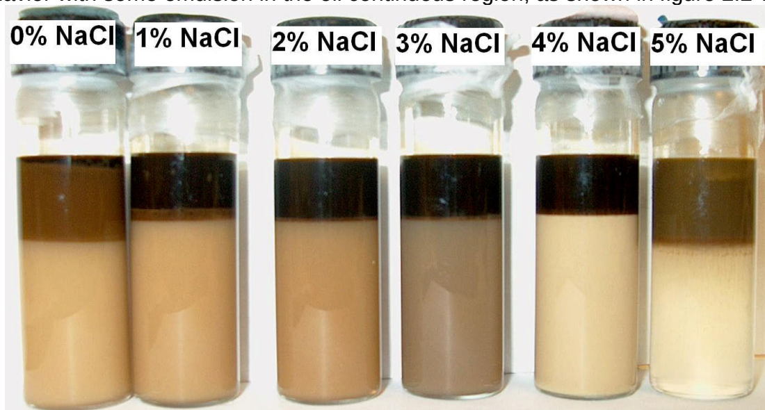
Figure 2.2-12 Phase behavior of 0.2% NI blend/1% Na 2 CO 3 (24 hours mixing, 4 hours settling)
