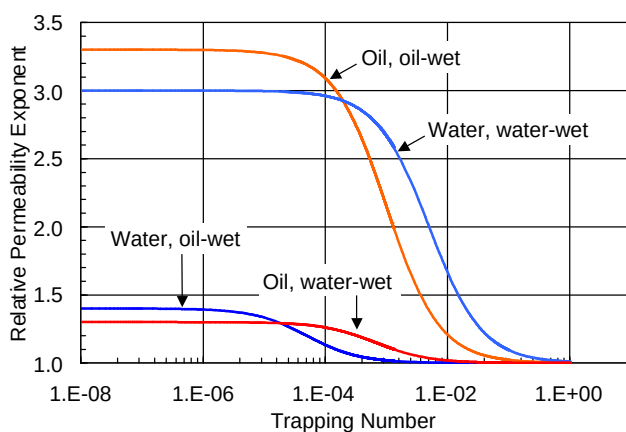
Fig. 4.1-3 Relative Permeability Exponent.
