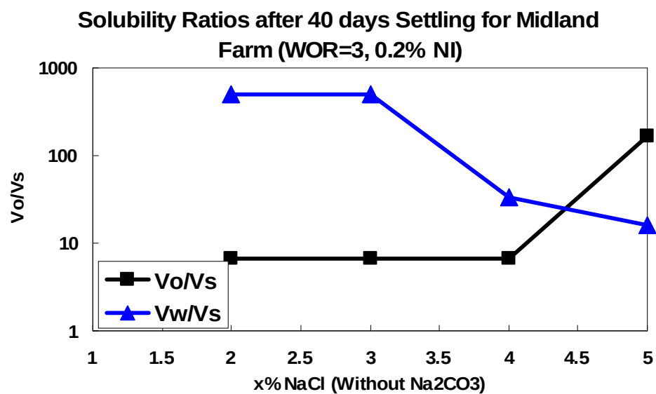
Figure 2.5-6 Solubility ratios for salinity scan of 0.2% NI / 0% \text{Na}_2\text{CO}_3 / x% NaCl
