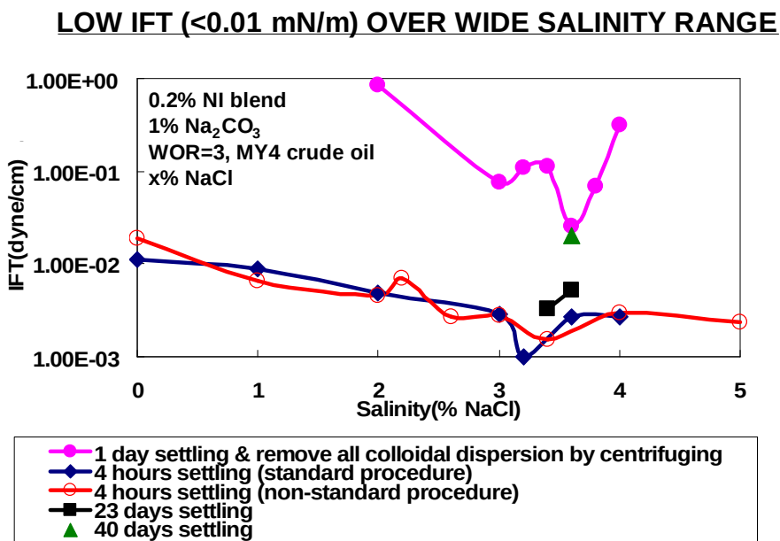
Figure 2.2-19 IFT change with salinity for 0.2NI-1%Na 2 CO 3 /WOR=3
