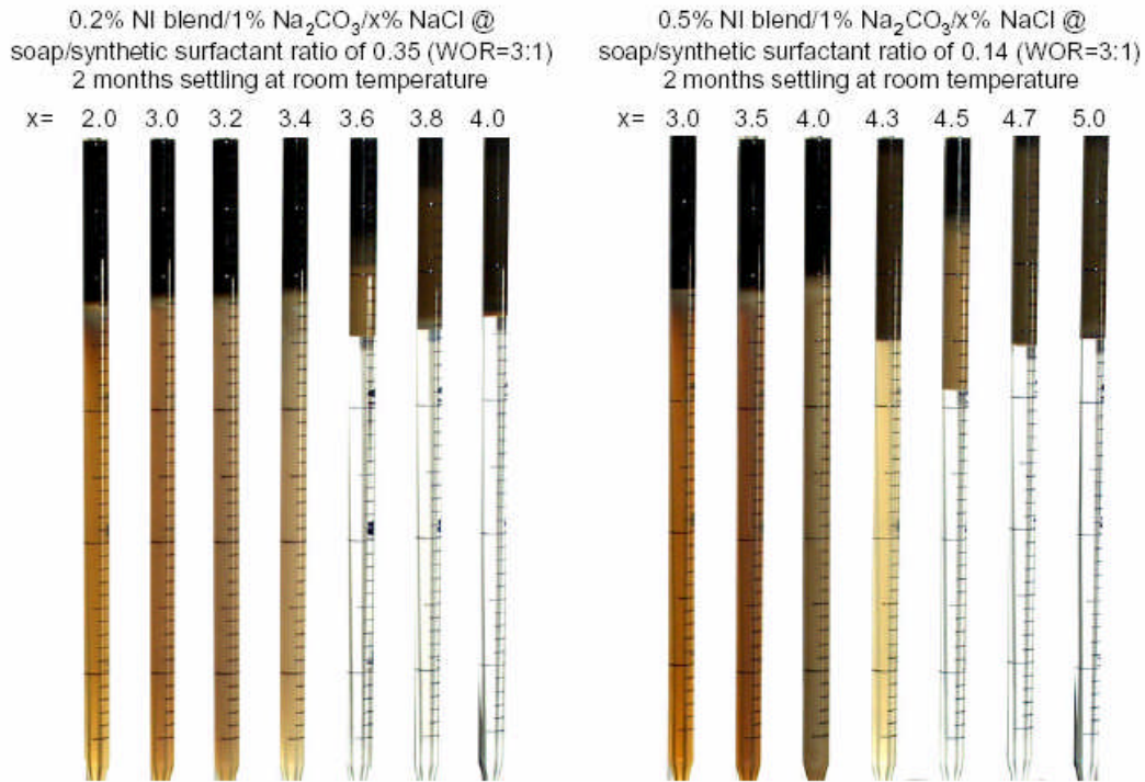
Figure 2.2-20 Phase behavior after 2 months with 0.2% and 0.5% NI blend.
