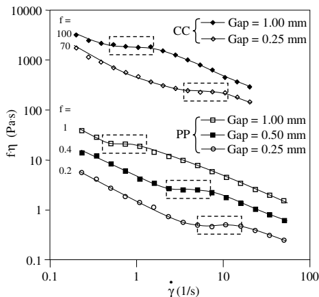
FIG. 2. Effect of gap on shear viscosity of emulsions with \phi = 0.58 for two geometries. The plots are shifted by a factor of f (indicated for each curve) to facilitate interpretation.
