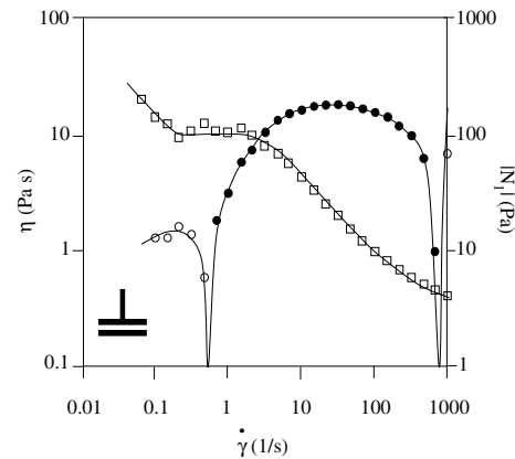
FIG. 3. Shear viscosity (squares) and magnitude of the first normal stress difference (circles) vs shear rate in an emulsion with \phi = 0.58 (parallel-plate geometry, gap = 0.65 mm). Filled circles indicate negative N_1 .
