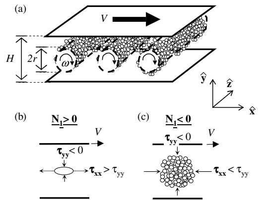
FIG. 5. Schematic representation of (a) the conformation of cylindrical flocs and (b), (c) the stresses in the plane of shear.
