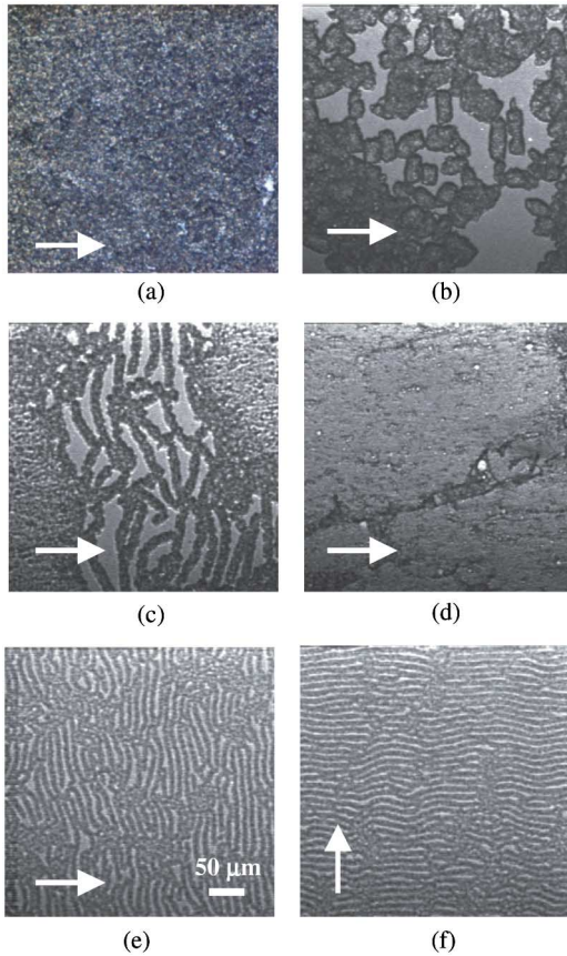
FIG. 4 (color online). Microphotographs of emulsions with \phi = 0.58 under simple shear for gap thicknesses of (a)–(d) 20 \mu\text{m} and (e), (f) 12 \mu\text{m} . Arrows indicate the direction of shear. The reference scale for all frames is inserted in frame (e).
