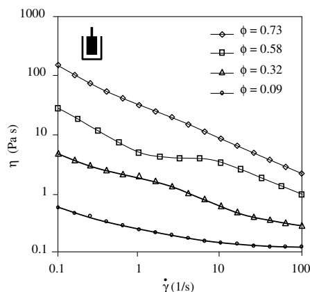
FIG. 1. Steady shear viscosity of water-in-oil attractive emulsions at several water contents (large concentric cylinders).
