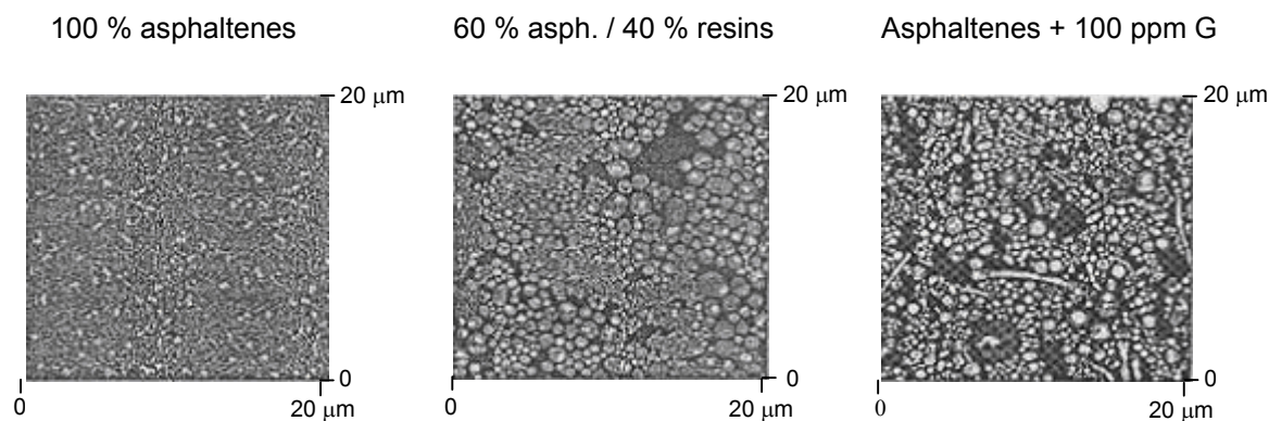
Figure 4.8. Langmuir-Blodgett films of asphaltenes, asphaltenes + resins and asphaltenes + high molecular weight demulsifier (G) at the water/air interface, studied by means of atomic force microscopy (AFM). Resins and demulsifier modify the structure of the asphaltene film in a similar fashion [28].
