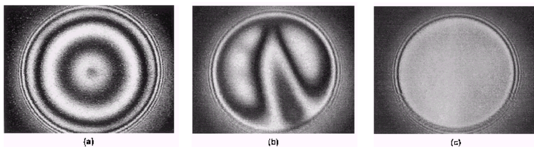
Figure 1.7. Upper view of interference patterns observed in the drainage of a thin film of a toluene diluted bitumen film in water. (a) drainage is axisymmetrical when the dimple is formed; (b) an instability develops and the drainage takes place asymmetrically; (c) an equilibrium gray film is obtained at the end. The film remained stable over one hour before break-up [40].
