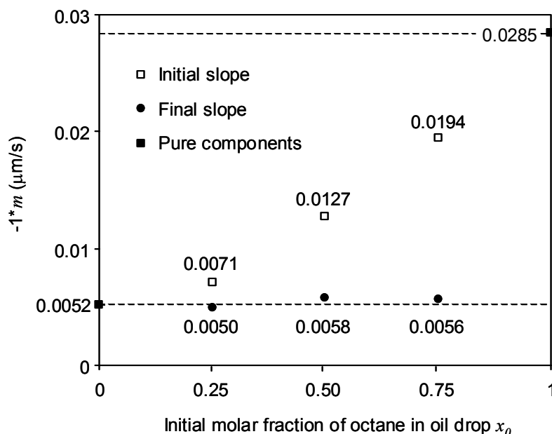
Figure 2.14. Experimental values for the initial and final rates of decay of drop radius of mixed drops of n-octane and n-undecane in an oil-free solution of \text{C}_{12}\text{E}_8 (2.5 wt. %) in water ( \theta = 0 ) at 30.9 °C.
