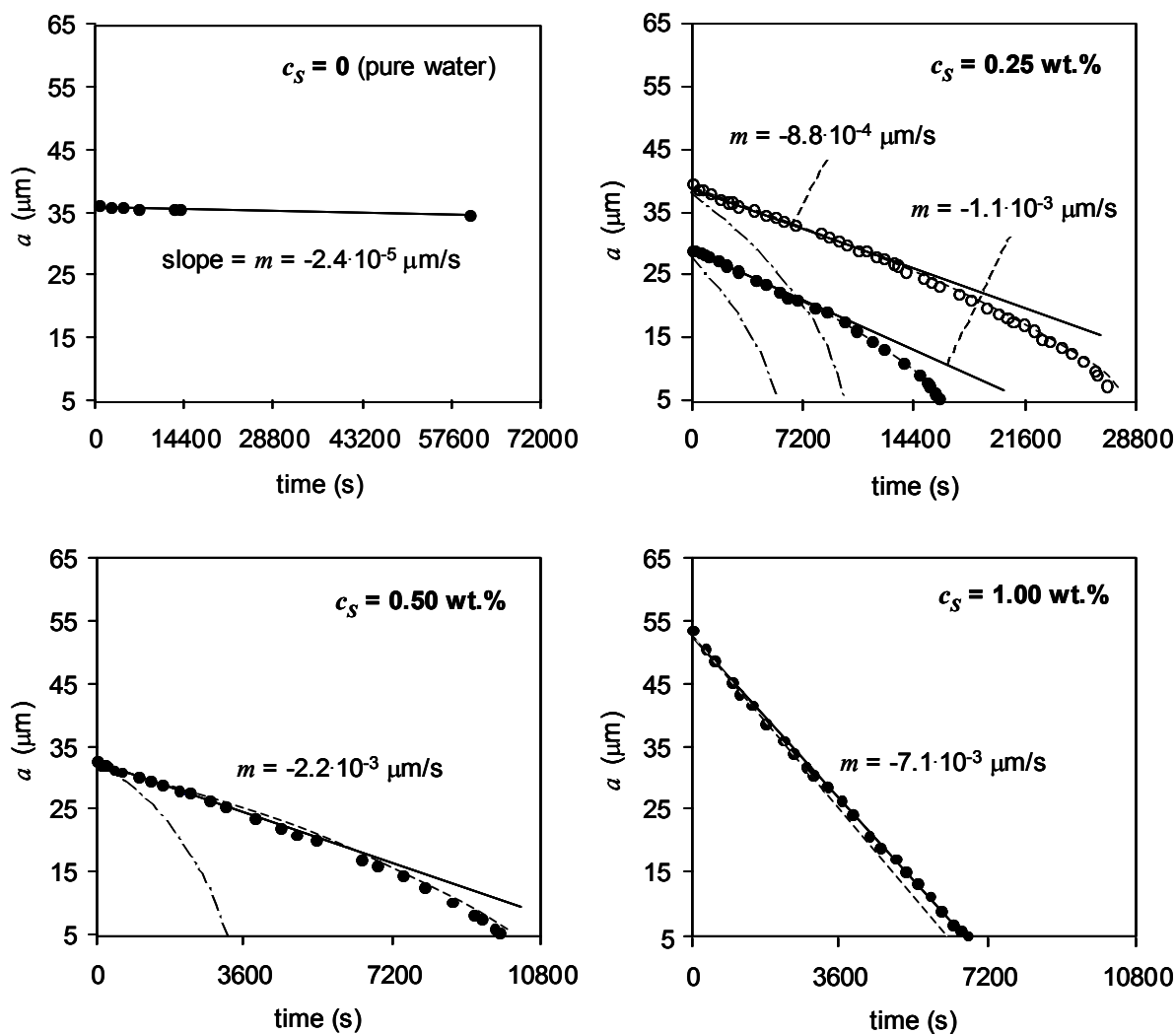
Figure 2.29. Solubilization of drops of n-octane in oil-free aqueous solutions of C_{12}E_8 at several surfactant concentrations. All experiments were performed at 30.9 \pm 0.1 °C. Symbols, experimental data. Solid lines, linear fit of the data (only first six points for the data for experiments at 0.25 wt.% and 0.5 wt.% C_{12}E_8 ). The slopes that are reported correspond to the solid lines. Dash-dot lines, predicted trend assuming micellar diffusion as rate-controlling. Dashed lines, predicted trends assuming mixed kinetics and considering spontaneously-generated convection as the surfactant concentration is increased. C_{12}E_8 concentration: 1.00 wt.% = 18.60 \text{ mol/m}^3 . (Figure continues on next page).
