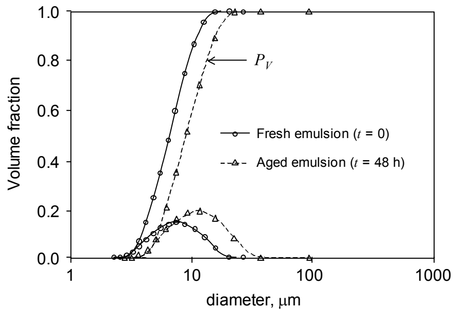
Figure 3.11. NMR results for the drop size distribution of fresh ( t = 0 ) and aged ( t = 48 h) emulsions of water (30 vol.%) in SHU.
