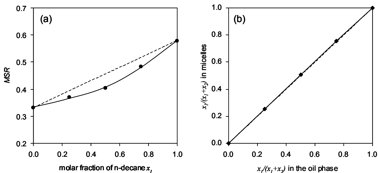
Figure 2.12. (a) Molar solubilization ratio, and (b) composition of oil and micellar phases in equilibrium for the n-decane/n-undecane system in solutions of C_{12}E_8 (2.5 wt.%) at 30.9°C [50].
