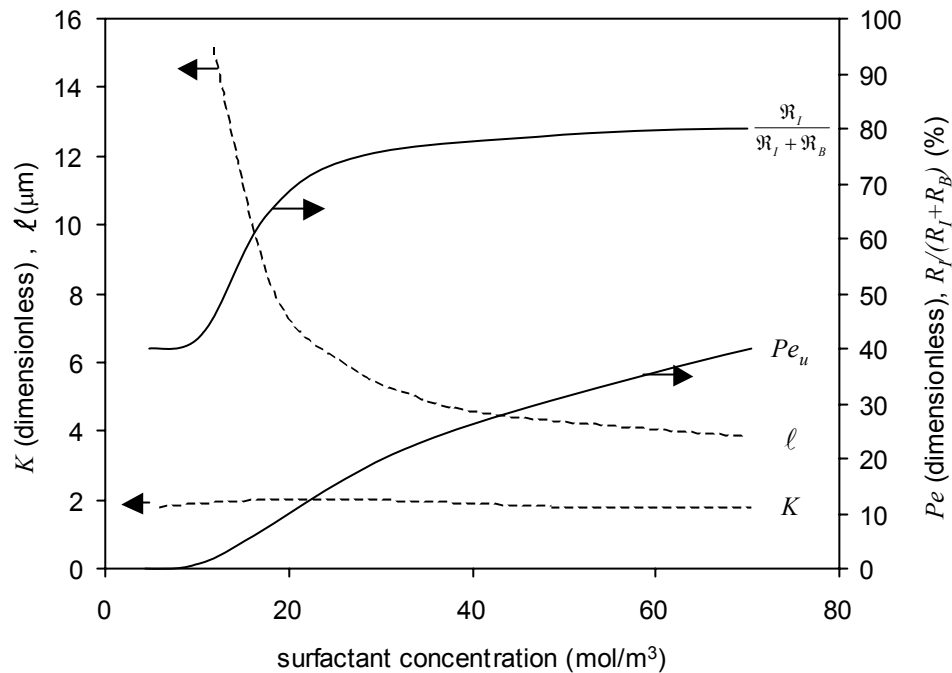
Figure 2.35. Effect of surfactant concentration on K , Pe_u , \ell and \mathfrak{R}_I/(\mathfrak{R}_I + \mathfrak{R}_B) for the solubilization of n-octane in C_{12}E_8 aqueous solutions at 30.9 °C.
