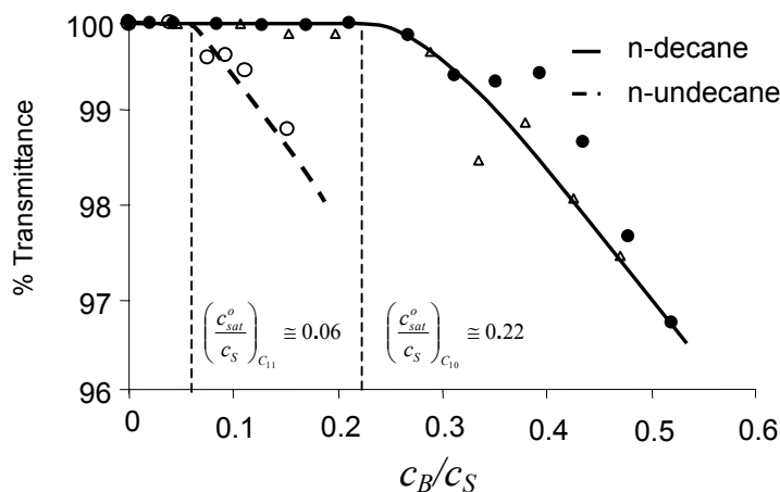
Figure 2.4. Light transmittance of aqueous C_{12}E_8 (2.5 wt.%) titrated with n-decane and n-undecane at room temperature. Triangles: Data obtained for n-decane allowing 4 hours between additions. Dots: Data obtained for n-decane allowing 10 hours between additions. Circles: Data for n-undecane allowing 10 hours between additions. The onset of a permanent turbidity indicates the solubility limit.
