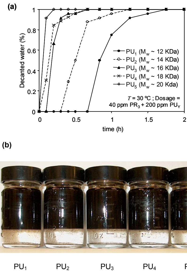
Figure 4.20. Effect of the molecular weight of the cross-linked polyurethane (200 ppm) on the transient amount of water separated in bottle tests, when dosed along with the phenolic resin PR 3 (40 ppm); (b) appearance of the samples one week after the beginning of the test.
