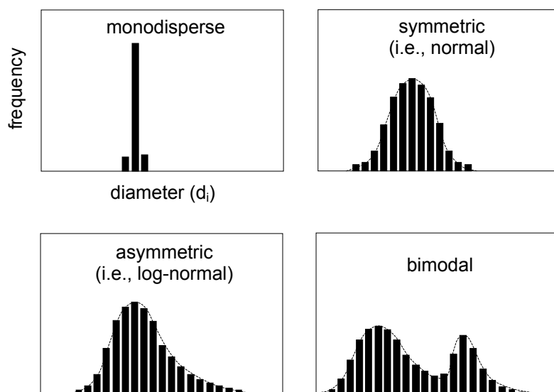
Figure 1.2. Drop size distributions commonly found in emulsions.
