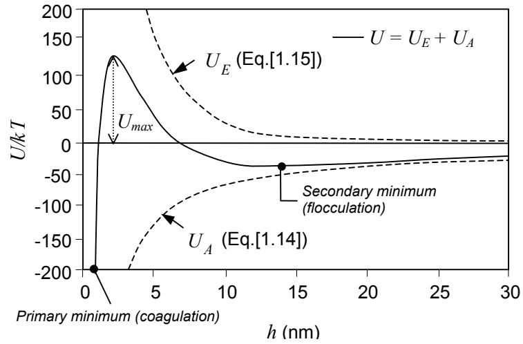
Figure 1.4. Energy of interaction between two spherical particles, as calculated from the DLVO theory. Parameters: droplet radius a = 3 \mu\text{m} , Hamaker constant A = 10^{-20} \text{ J} , surface potential \psi_0 = 60 \text{ mV} , Debye length 1/\kappa = 3 \text{ nm} ( c_0 = 10 \text{ mM} ) and T = 25^\circ\text{C} .
