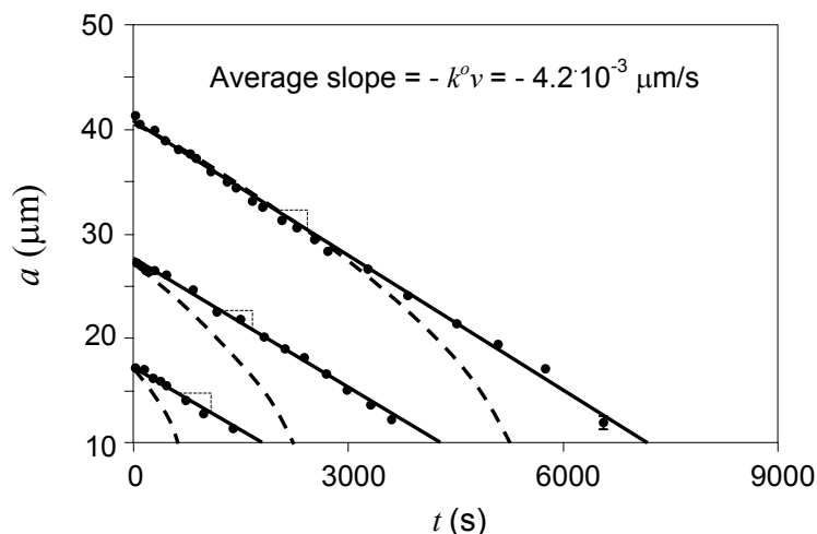
Figure 2.6. Solubilization of several drops of n-decane in an oil-free solution of C_{12}E_8 (2.5 wt. %) in water ( \theta^\circ = 0 ) at room temperature. Solid lines: linear fit of the data with Eq. [2.69]. Dashed line: predicted trend assuming mass transport controlled by micellar diffusion (Eq. [2.70]). Experimental error is shown in the last datum for the drop with largest initial radius.
