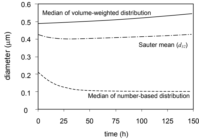
Figure 2.19. Case study 1: Numerical results for the transient behavior of the transient mean and Sauter drop sizes.
