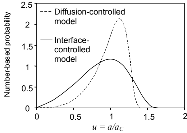
Figure 2.3. Plots of the asymptotic solutions for the number-based drop size distribution of emulsions undergoing Ostwald ripening.
