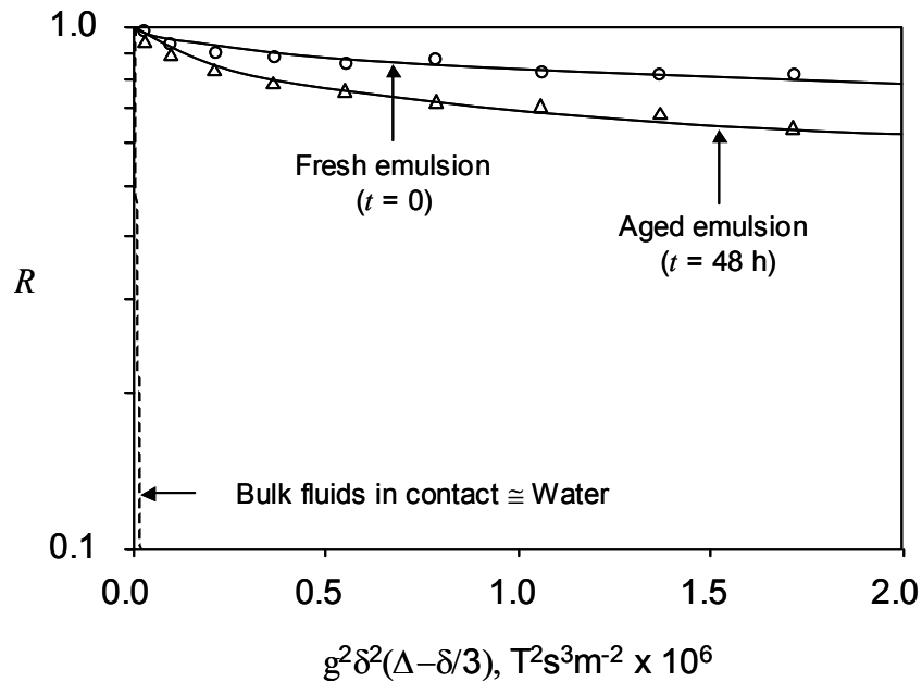
Figure 3.10. PGSE data for fresh ( t = 0 ) and aged ( t = 48 h) emulsions of water (30 vol.%) in crude oil SHU.
