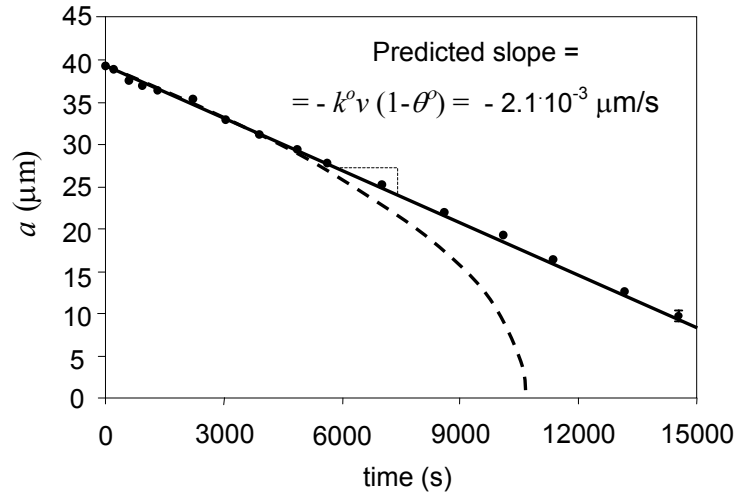
Figure 2.7. Solubilization of a drop of n-decane in aqueous C_{12}E_8 (2.5 wt. %) partially saturated with n-decane ( \theta^o = 0.50 ). Solid line: predicted trend assuming interfacial resistance as limiting (Eq. [2.69]). Dashed line: predicted trend when micellar diffusion is limiting (Eq. [2.70]).
