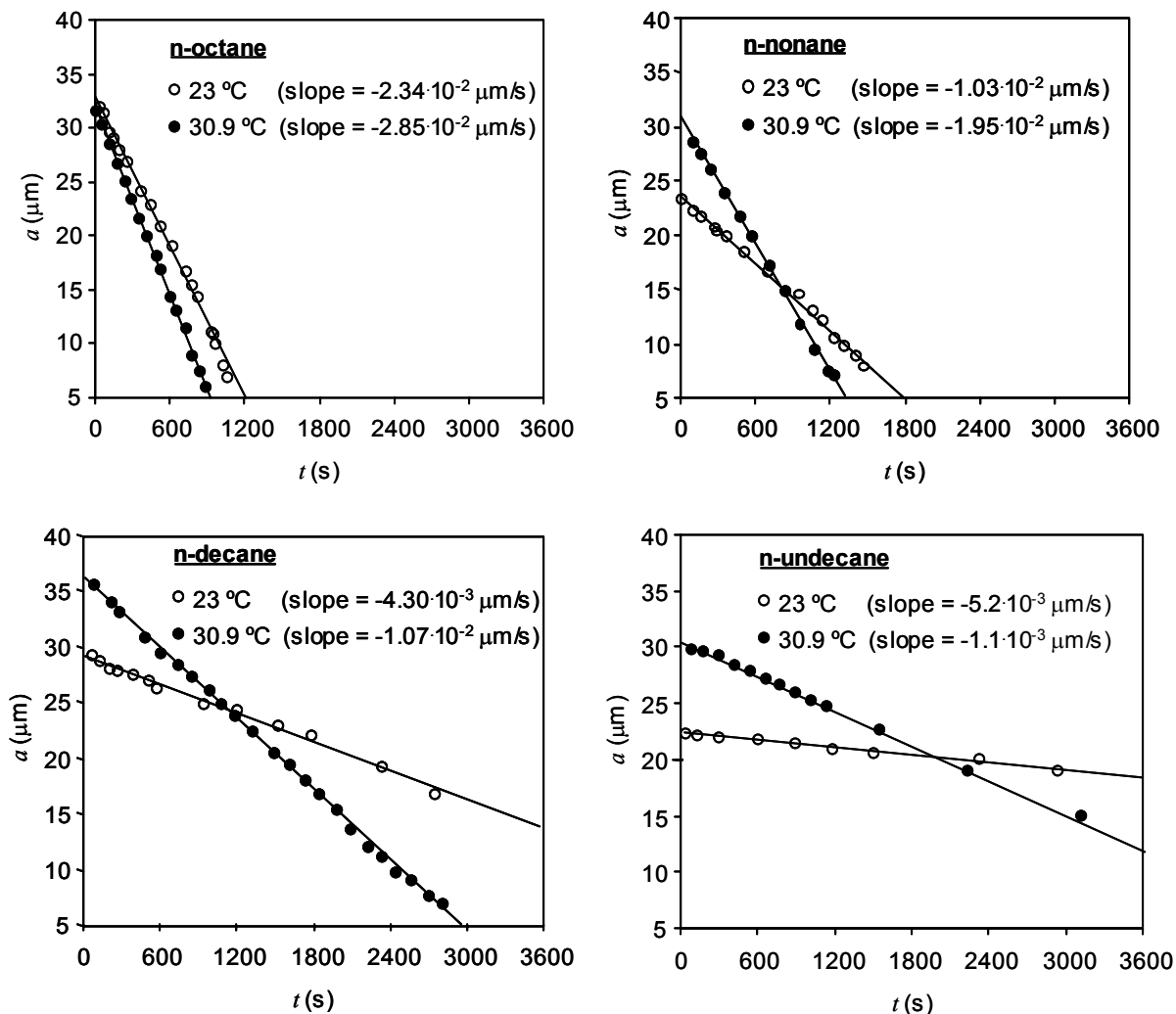
Figure 2.5. Solubilization of several drops of linear alkanes in oil-free solutions of \text{C}_{12}\text{E}_8 (2.5 wt.%) in water ( \theta^p = 0 ) at two different temperatures.
