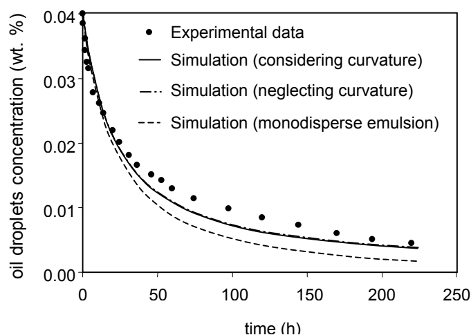
Figure 2.20. Case study 1: Experimental and numerical results for the concentration of oil present as droplets in the emulsion.
