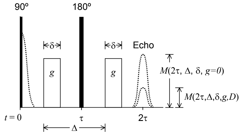
Figure 3.2. Sequence of events in a PGSE experiment.
