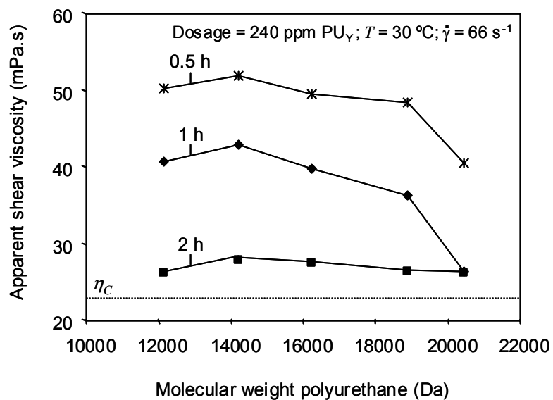
Figure 4.18. Effect of the molecular weight of the polyurethanes on the transient behavior of the shear viscosity.
