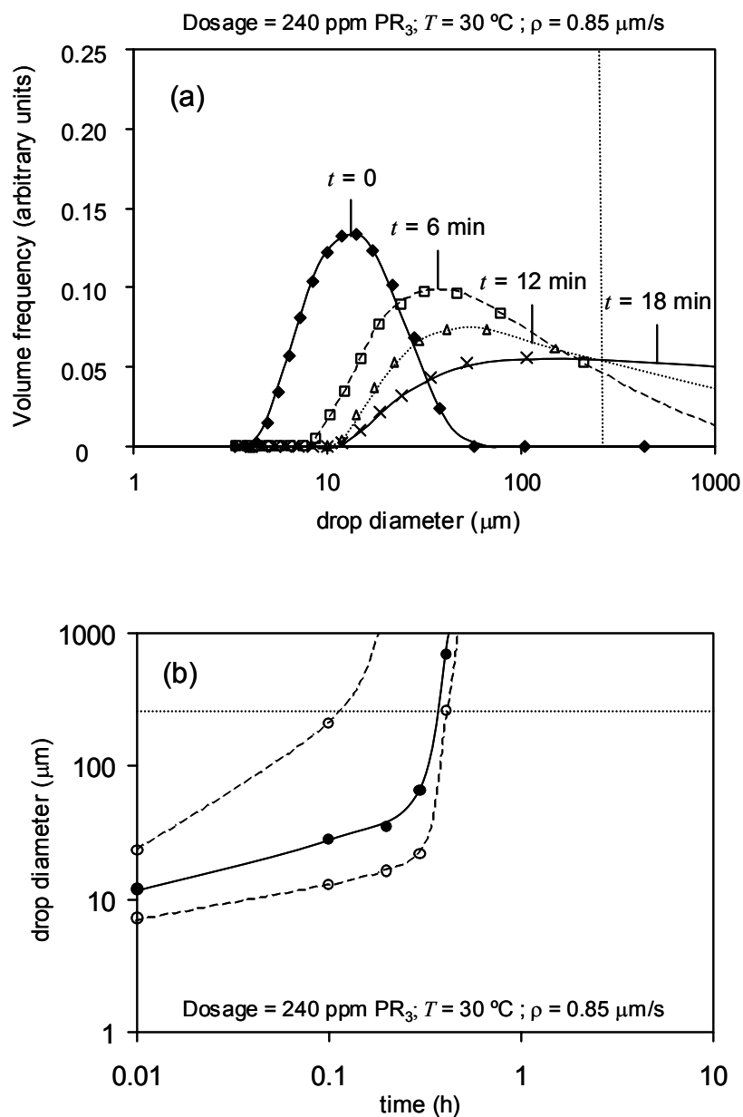
Figure 4.27. (a) Time-dependent drop size distribution of the emulsion treated with 240 ppm of phenolic resin \text{PR}_3 ; (b) transient behavior of the Sauter mean diameter d_{AV} (filled circles) and polydispersity (open circles) of the emulsion. The convention used to calculate the lower and upper limits shown in open circles is provided in the text.
