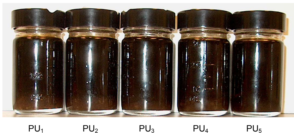
Figure 4.17. Appearance of the samples used in the bottle tests with the cross-linked polyurethanes PU_Y (240 ppm), five months after the beginning of the test.
