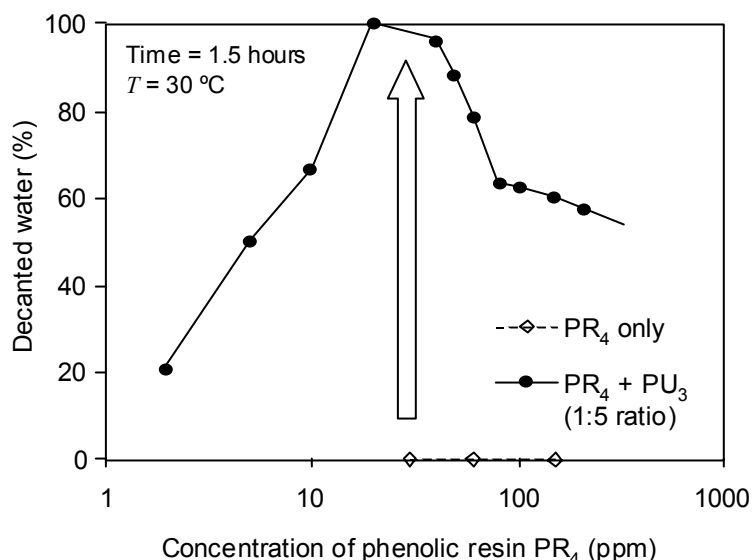
Figure 4.24. Results from bottle tests for emulsions treated with the phenolic resin PR 4 with (filled circles) and without (open circles) polyurethane PU 3 . The arrows illustrate synergistic and inhibiting effects on the performance.
