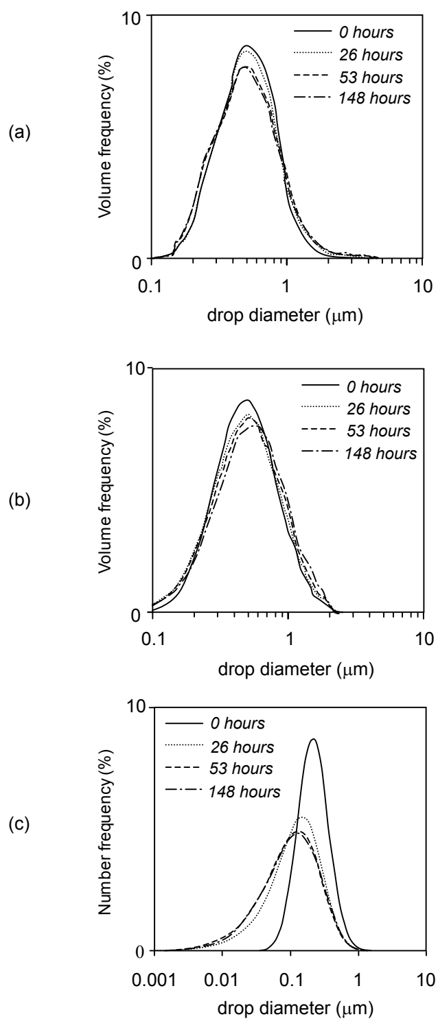
Figure 2.18. Case study 1: [(a)] Experimental data and [(b), (c)] simulation results for the transient volume (b) and number (c) drop size distribution of the emulsion.
