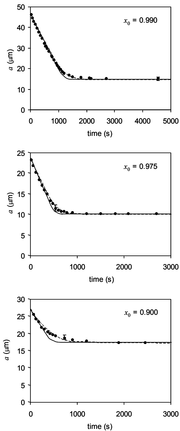
Figure 2.10. Solubilization of mixed drops of n-octane and squalane in an oil-free solution of C 12 E 8 (2.5 wt. %) in water ( \theta^\circ = 0 ) at 30.9 °C. Solid lines: predicted trends assuming mass transport controlled by interfacial resistance and \mathbf{a}_j = x_j . Dashed lines: predicted trends assuming mass transport controlled by interfacial resistance and \mathbf{a}_j = \phi_j .
