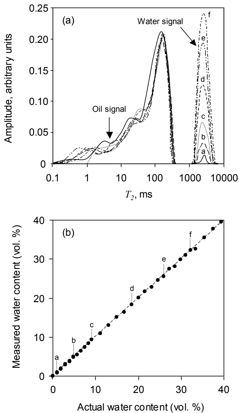
Figure 3.19. Determination of water composition via CPMG. (a) T_2 distribution of selected emulsions of water in SHU. Data were normalized with respect to the oil signal; (b) comparison between actual and NMR-measured water contents.
