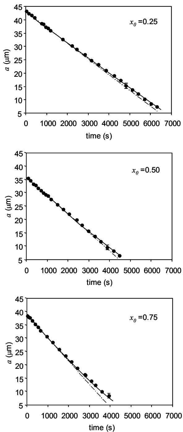
Figure 2.16. Solubilization of mixed drops of n-decane and n-undecane in oil-free solutions of \text{C}_{12}\text{E}_8 (2.5 wt. %) in water ( \theta = 0 ) at 30.9^\circ\text{C} . Dots: Experimental data. Solid lines: Predictions from multicomponent mass transfer model assuming interface-controlled mass transfer. Dash-dot lines, Predictions assuming that the initial solubilization rate remains constant.
