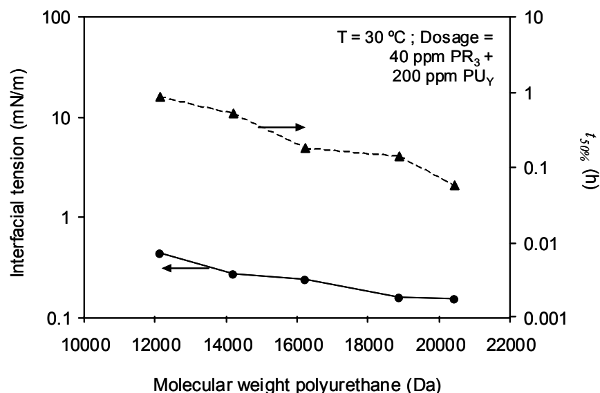
Figure 4.21. Effect of the molecular weight of the cross-linked polyurethane on the equilibrium interfacial tensions of emulsions treated with \text{PU}_\gamma (200 ppm) and 40 ppm of phenolic resin \text{PR}_3 (filled circles). The times required in bottle tests to decant 50 % of the brine initially present in the emulsion are also plotted (triangles).
