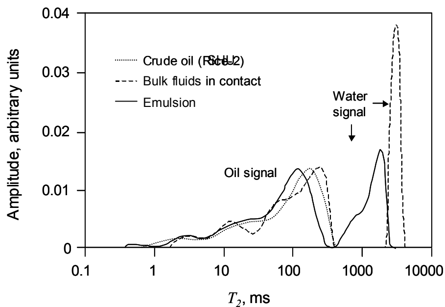
Figure 3.13. T_2 distribution of a blend of two emulsions of water (30 vol.%) in SHU.
