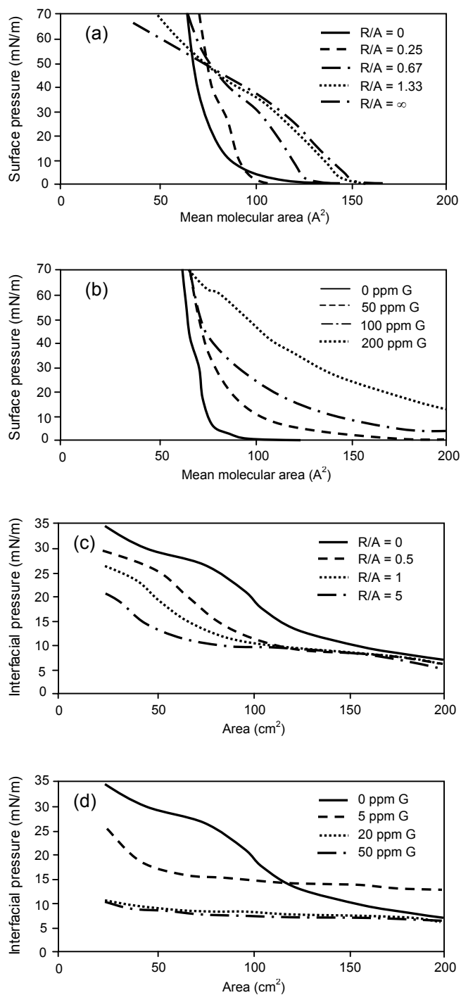
Figure 4.7. \Pi -A isotherms for (a) asphaltene/resins mixtures at the air/water interface; (b) asphaltene/demulsifier (G) mixtures at the air/water interface; (c) asphaltene/resins mixtures at the oil/water interface; (d) asphaltene/demulsifier mixtures at the oil/water interface.
