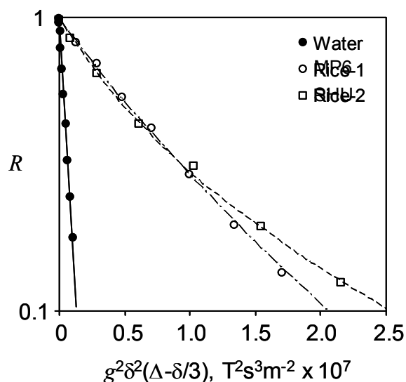
Figure 3.4. PGSE data for water and crude oils MP6 and SHU.
