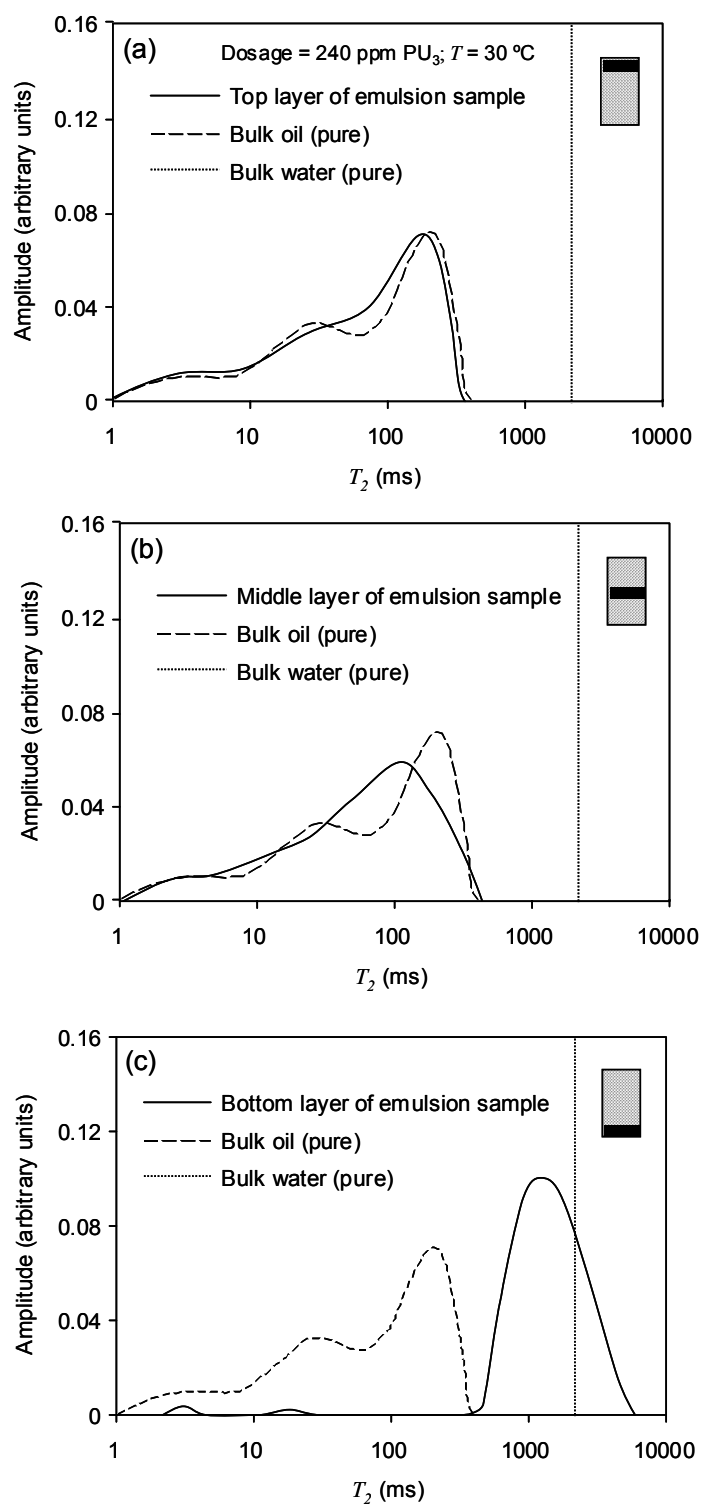
Figure 4.31. T_2 distributions of selected regions of the emulsion treated with 240 ppm of cross-linked polyurethane \text{PU}_3 , one week after the beginning of the experiment.
