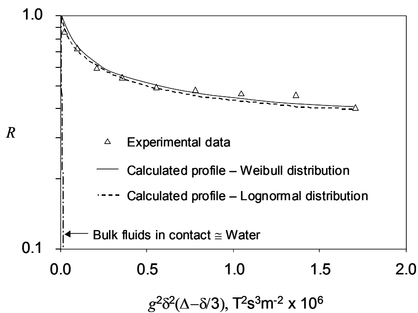
Figure 3.14. PGSE data for the blend of two emulsions of water (30 vol.%) in SHU.
