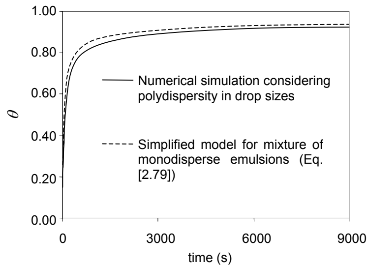
Figure 2.28. Case study 3: Transient behavior of the concentration of n-decane in the surfactant solution, expressed in dimensionless form \theta^o = c_B^o / c_{sat}^o
