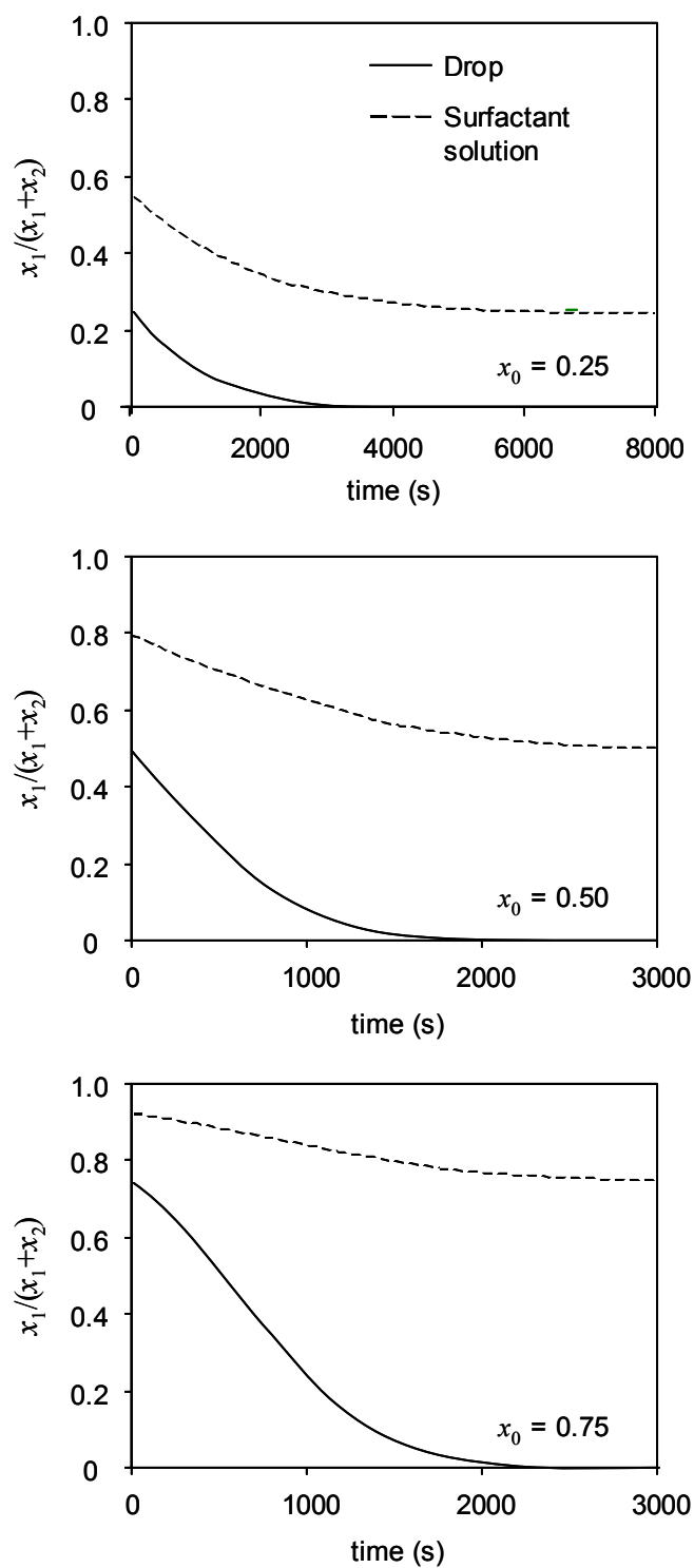
Figure 2.15. Predicted trends for the molar composition x_1/(x_1+x_2) of the oil drops and surfactant solutions for the solubilization of mixtures of n-octane (1) / n-undecane (2) in C_{12}E_8 (2.5 wt.%) at 30.9 °C.
