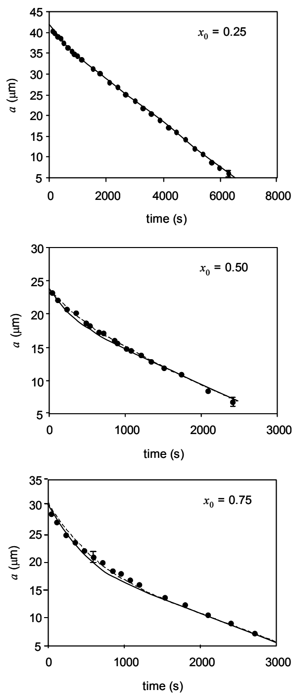
Figure 2.13. Solubilization of mixed drops of n-octane and n-undecane in an oil-free solution of C 12 E 8 (2.5 wt. %) in water ( \theta^o = 0 ) at 30.9 °C. Solid lines: predicted trends assuming mass transport controlled by interfacial resistance and \mathbf{a}_j = x_j . Dashed lines: predicted trends assuming mass transport controlled by interfacial resistance with the experimental activities reported in Figure 2.12.
