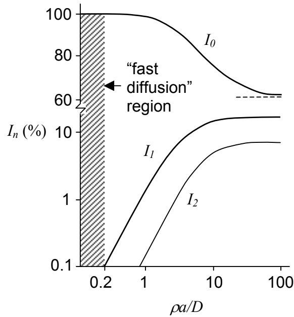
Figure C.1. Plot of the three first intensities I_0 , I_1 and I_2 of the magnetization of an isotropic fluid confined in a sphere. In the “fast diffusion” mode, the first intensity I_0 dominates. Adapted from Ref. [1]
