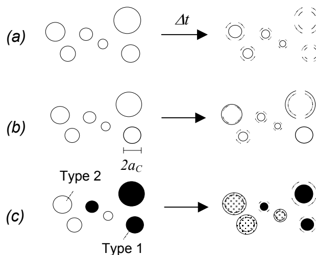
Figure 2.1. Schematic representations showing the transient behavior of drops sizes in emulsions undergoing mass transfer. (a) Solubilization of drops in an undersaturated surfactant solution: as time proceeds, a reduction in the sizes of the droplets is expected; (b) Ostwald ripening: drops with radii a(t) greater than a critical size a_c(t) grow, while those with a(t) < a_c(t) shrink; (c) compositional ripening in a mixed emulsion containing two drop types, with one of them (white circles) being insoluble in the surfactant solution: the latter grow at the expense of the solubilization of drops containing a soluble solute (black circles).
