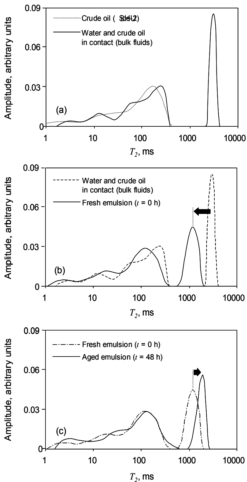
Figure 3.9. T_2 distribution of mixtures of water (30 vol.%) and SHU, contacted as bulk fluids and emulsified.
