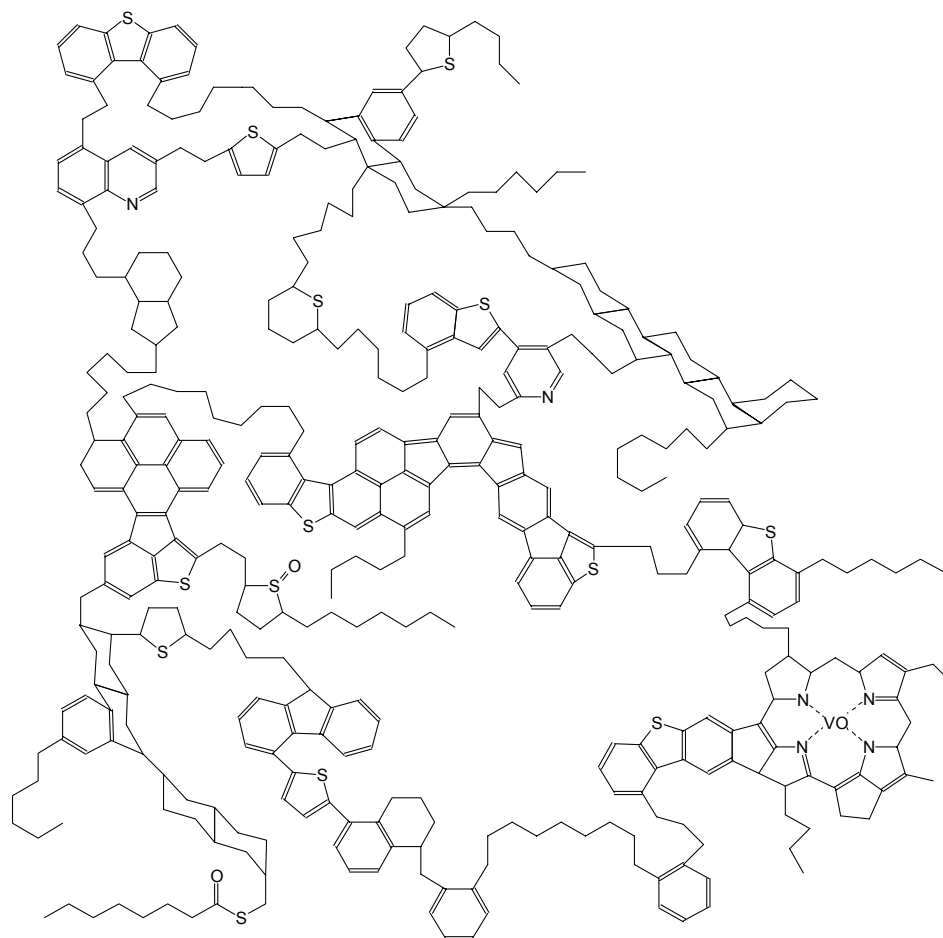
Figure 4.2. Proposed structure for asphaltenes in Athabasca bitumen [6].
