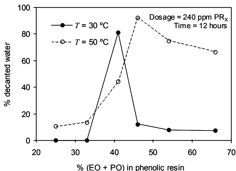
Figure 4.12. Effect of EO/PO content and temperature on the performance of the phenolic resins in bottle tests.
