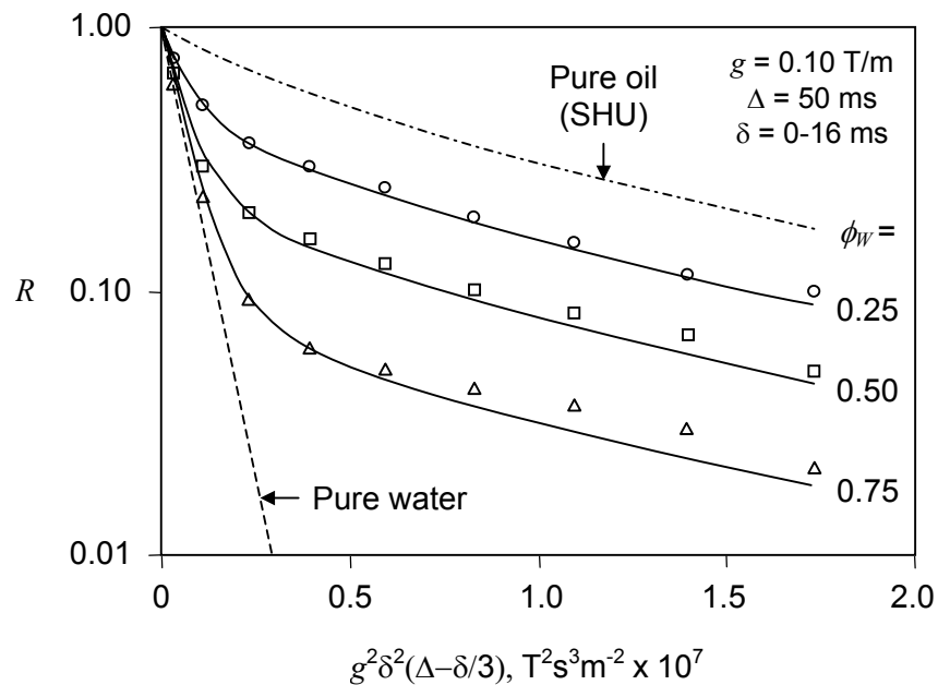
Figure 3.5. PGSE results for mixtures of water and SHU at several water-oil compositions. No parameters have been adjusted in the calculations and the comparison with the experimental data is absolute.
