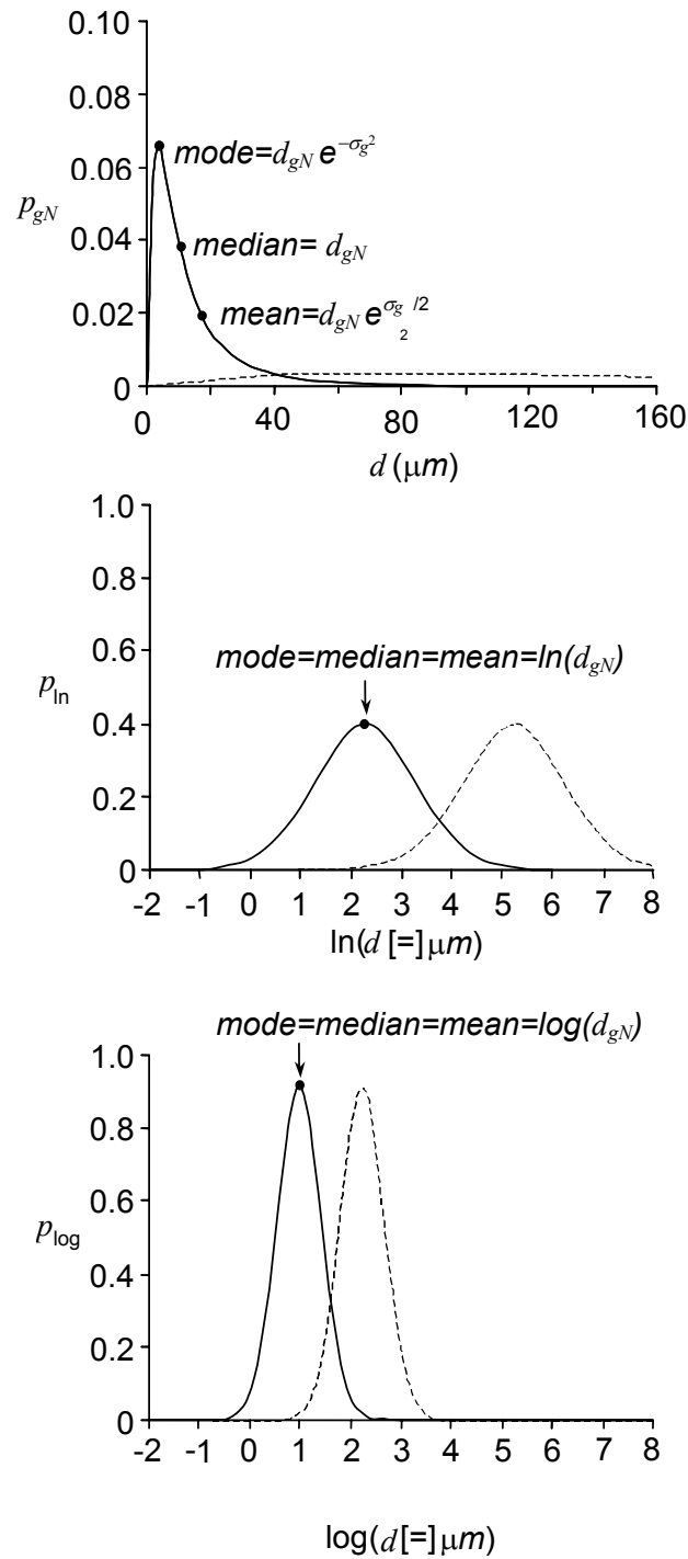
Figure A.1. Calculated log-normal size distributions as a function of the scale used to plot particle size, using d_{gN} = 10 \mu m and \sigma_g = 1 . Solid lines: number-based distributions. Dashed lines: corresponding volume-weighted distributions.
