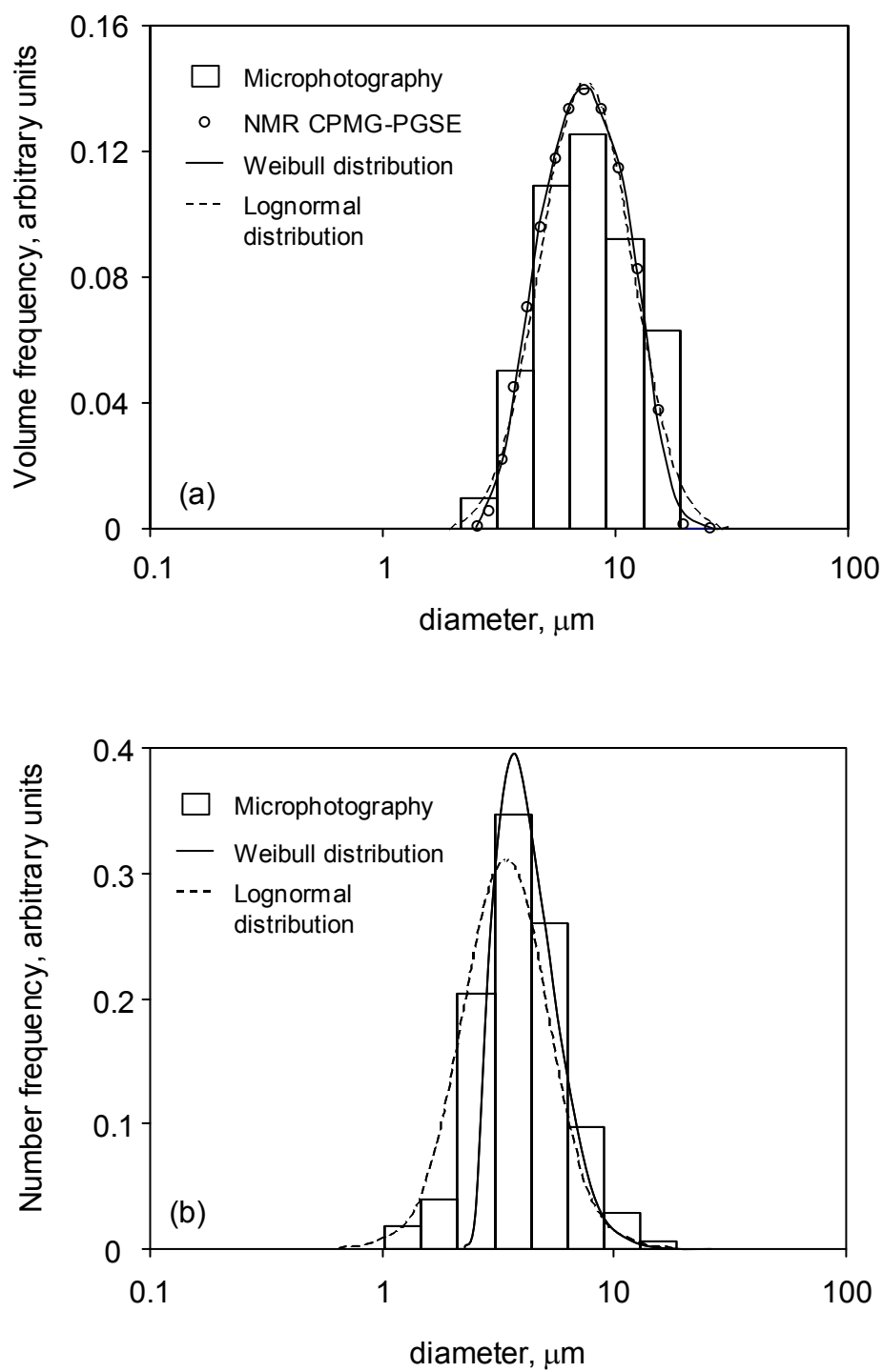
Figure 3.12. Drop size distribution of the fresh emulsion: Comparison of NMR and microphotography results. (a) Volume-weighted distribution; (b) number-based distribution.
