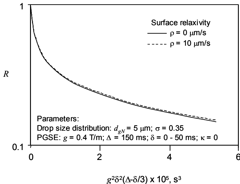
Figure 3.20. Simulated attenuation profiles at two different surface relaxations for a hypothetical W/O model emulsion at 25 °C.
