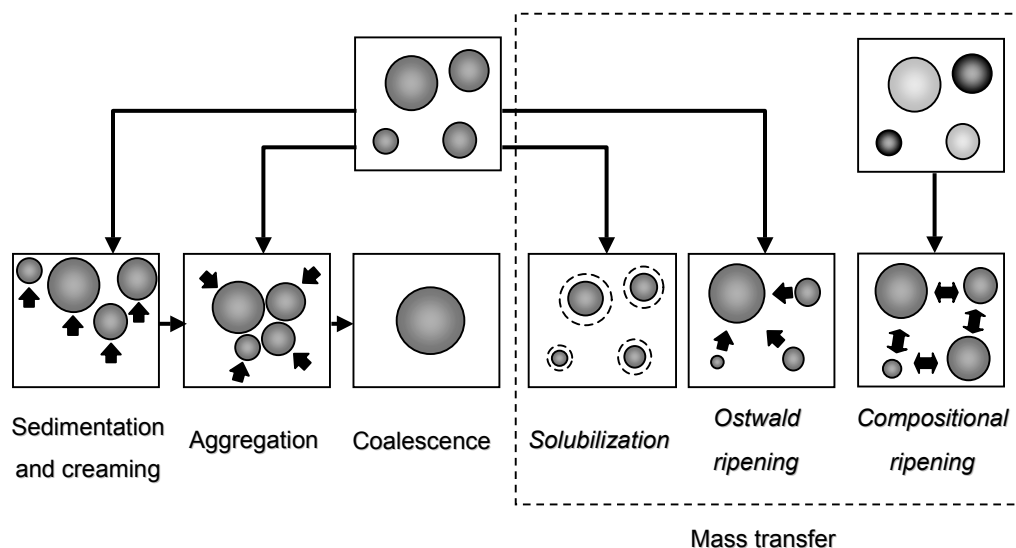
Figure 1.3. Destabilizing mechanisms in emulsions.
