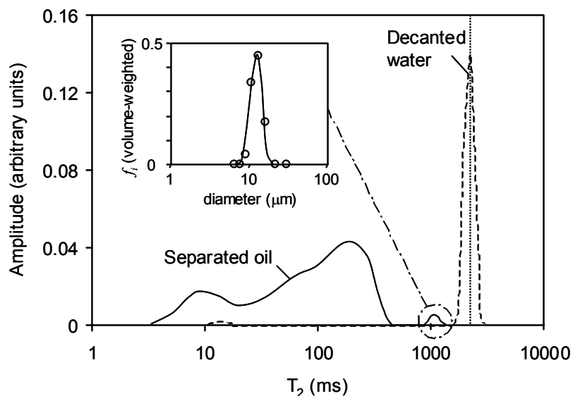
Figure 4.28. T_2 distributions of the oil and water phases that were separated by decantation from the emulsion treated with 240 ppm of phenolic resin PR 3 , one week after the beginning of the experiment. The inserted plot shows the estimated drop size distribution for the droplets that remained dispersed in the oil phase.
