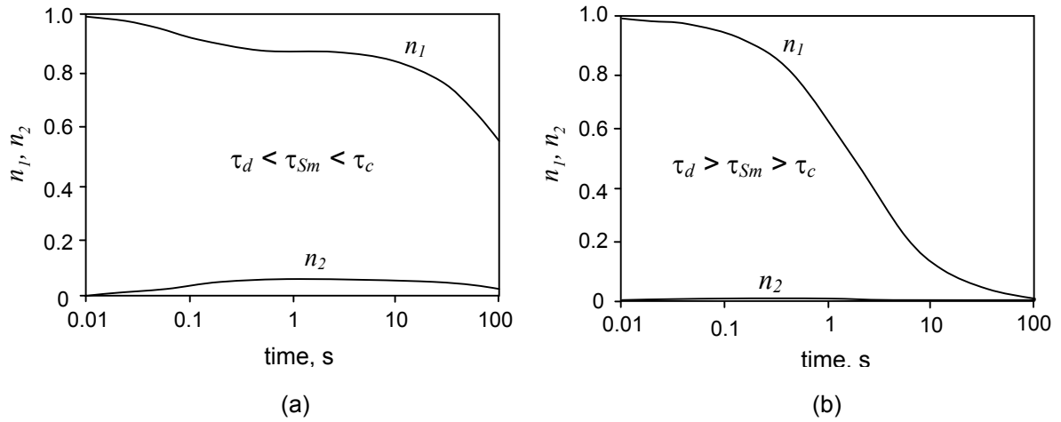
Figure 1.9. Time-dependent behavior of the concentration of single drops ( n_1 ) and doublets ( n_2 ) in a 5 vol. % O/W emulsion undergoing aggregation and coalescence. (a) fast aggregation, slow coalescence. (b) slow aggregation, fast coalescence. Parameters: T = 298 K, \eta = 1 mPa.s, a = 1 \mu\text{m} , ( \tau_{Sm} = 1.7 s) (a) U_{min} = -45kT ( \tau_d = 0.1 s), \tau_c = 10 s (b) U_{min} = -40kT ( \tau_d = 19.5 s), \tau_c = 0.01 s.
