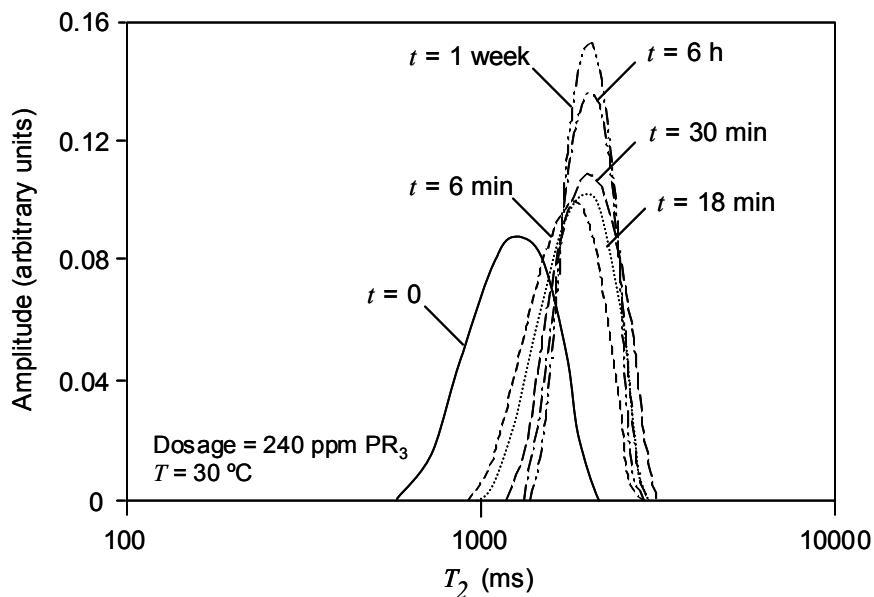
Figure 4.26. Evolution of the T_2 distribution of the water phase for an emulsion treated with 240 ppm of the phenolic resin PR_3 . The distribution of the oil phase has been omitted to simplify the interpretation of the plot.
