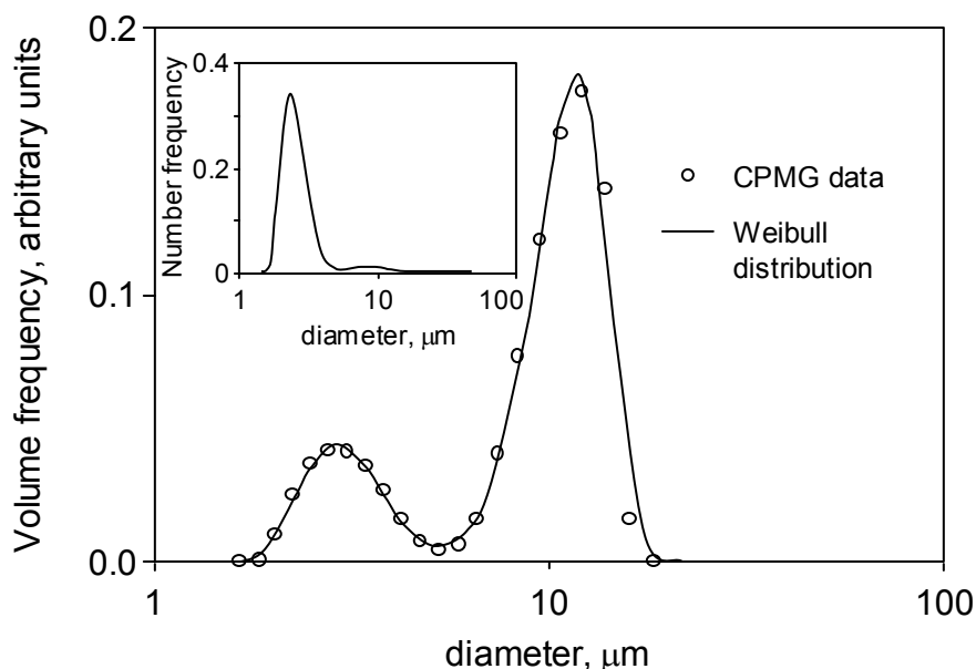
Figure 3.18. Volume-weighted and number-based drop size distribution of a bimodal
