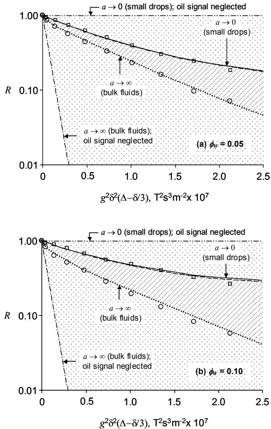
Figure 3.8. Effect of the transverse magnetization of the continuous phase on the PGSE response of mixtures of water and MP6, contacted as bulk fluids and emulsified. The features of the plot are explained in the text. (a) Mixtures with \phi_W = 0.05 ; (b) mixtures with \phi_W = 0.10 .
