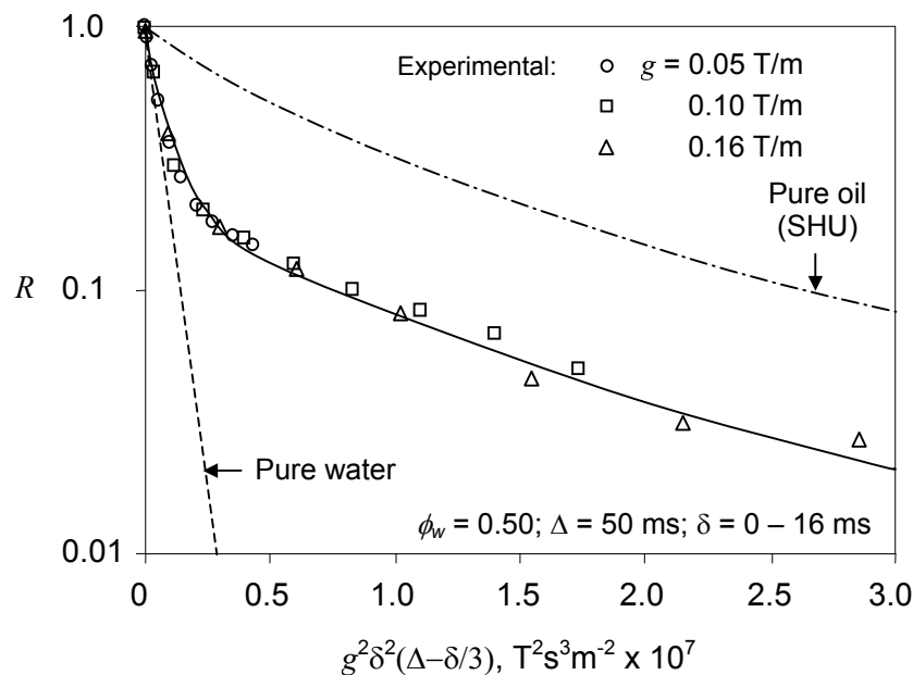
Figure 3.6. PGSE results for a mixture of water (50 vol.%) and SHU contacted as bulk fluid, not emulsified. Measurements were performed at different values of g .
