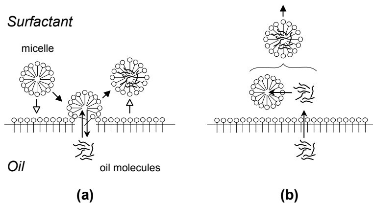
Figure 2.36. Schematic representation of plausible molecular mechanisms able to dictate interfacial resistance to mass transport. (a) Complete (white arrows) or partial (black arrows) adsorption of micelles, followed by emission/desorption; (b) molecular transport of solute, followed by irreversible incorporation in micelles.
