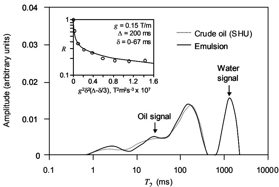
Figure 4.25. T_2 distribution of the emulsion used to follow-up the performance of demulsifiers via NMR. The inserted plot shows results from NMR-PGSE experiments for the same emulsion.
