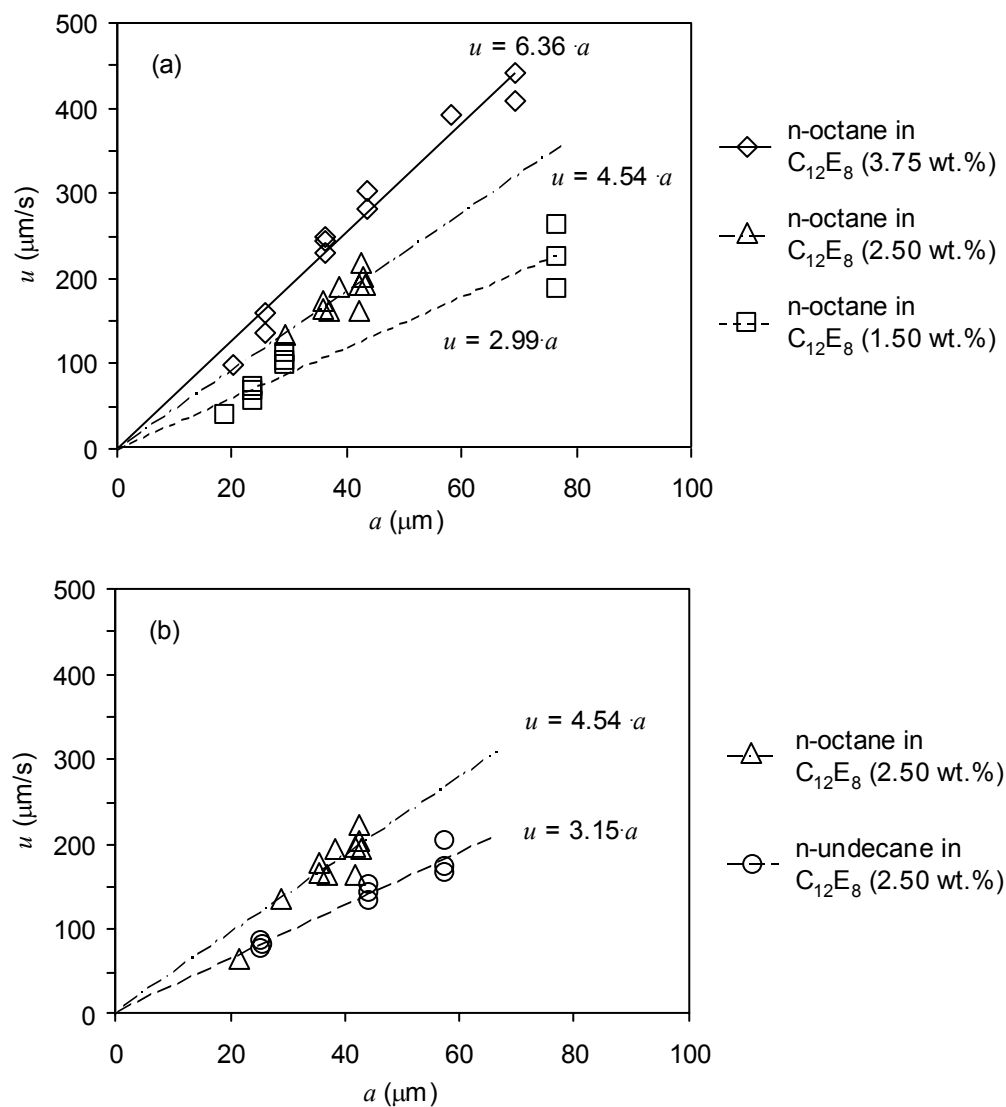
Figure 2.33. Effect of surfactant concentration, drop size and solubilized oil on the velocity of PS particles present in solubilization experiments.
