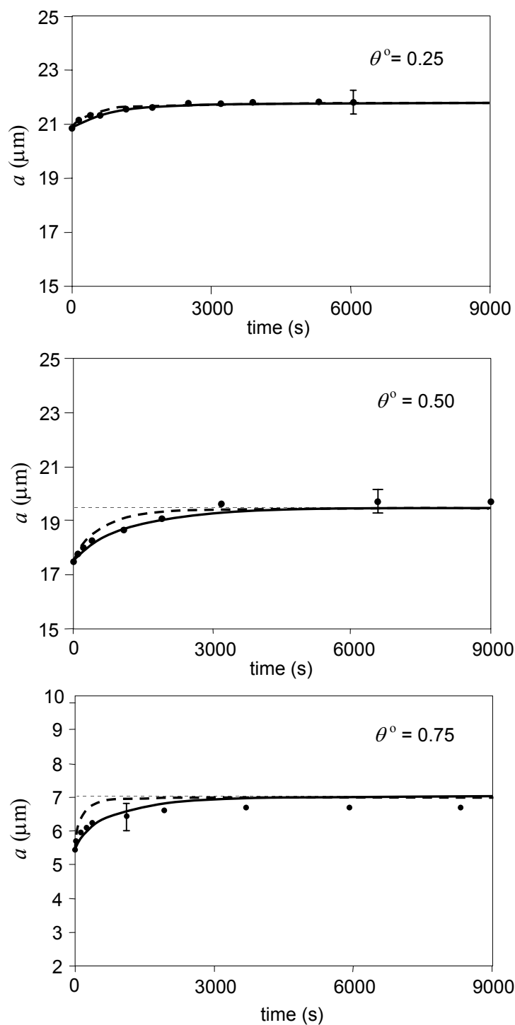
Figure 2.9. Swelling of drops of squalane in aqueous \text{C}_{12}\text{E}_8 (2.5 wt. %) partially saturated with n-decane at 23°C. Solid lines: predicted trends assuming interfacial phenomena as limiting (Eq. [2.8]). Dashed lines: predicted trends assuming micellar diffusion as limiting (Eq. [2.11]). Dotted lines: Predicted radii at equilibrium, determined from the condition x = \theta^0 .
