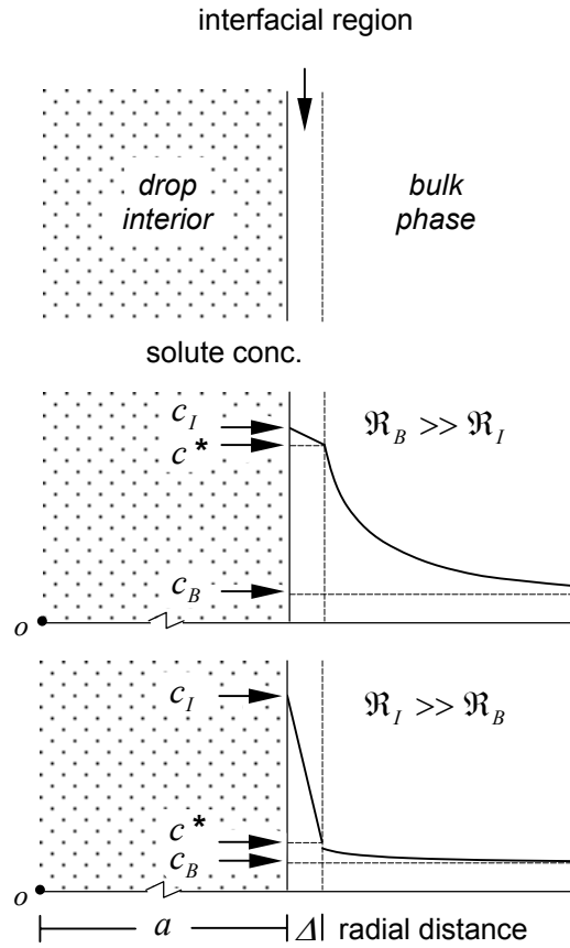
Figure 2.2. Basic configuration of the water-oil interfacial region showing the quasi-steady interface-controlled concentration profile of a solute being transferred from drop to solution.
