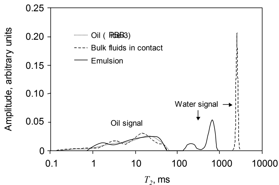
Figure 3.16. T_2 distribution of a bimodal emulsion of water (30 vol.%) in PBB.
