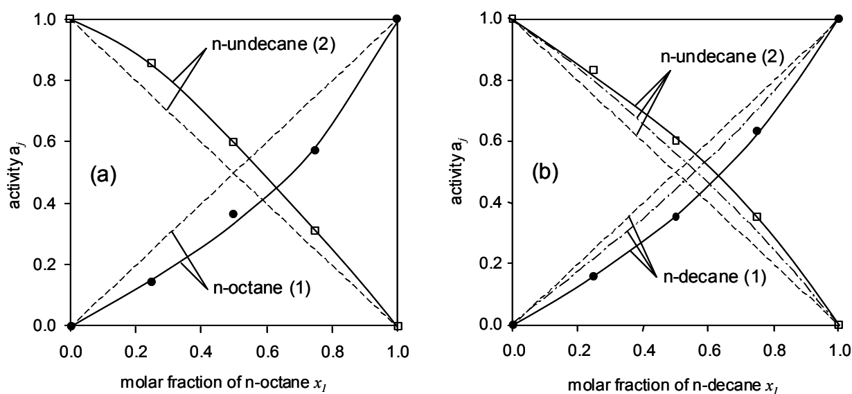
Figure 2.11. Measured activities ( a_j = c_{sat,j} / c_{sat,j}^o ) of individual components in n-octane/n-undecane and n-decane/n-undecane mixtures in contact with a solution of C_{12}E_8 (2.5 wt.%) at 30.9°C [50].
