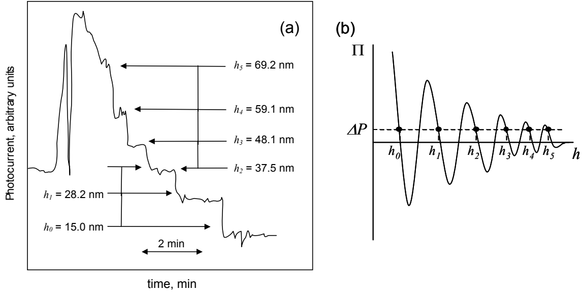
Figure 1.8. (a) Interferogram showing the stepwise thinning of a film of aqueous nonionic micellar solution (Adapted from Ref. [45]); (b) Schematic plot of the disjoining pressure \Pi vs. film thickness h . The equilibrium states of the liquid film correspond to \Pi = \Delta P , where \Delta P is the pressure difference across the film [37].
