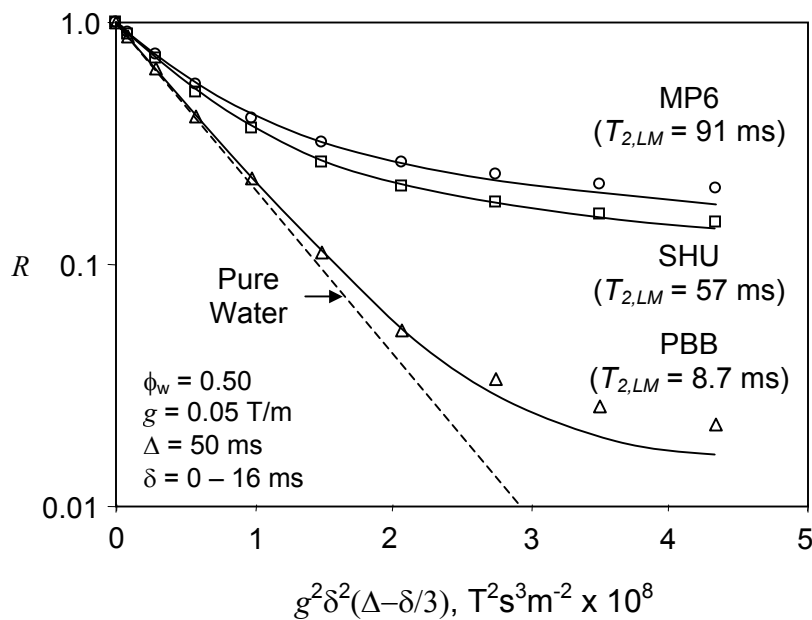
Figure 3.7. PGSE results for mixtures of water (50 vol.%) and MP6 (○), SHU (□) and PBB (Δ) contacted as bulk fluids, not emulsified.
