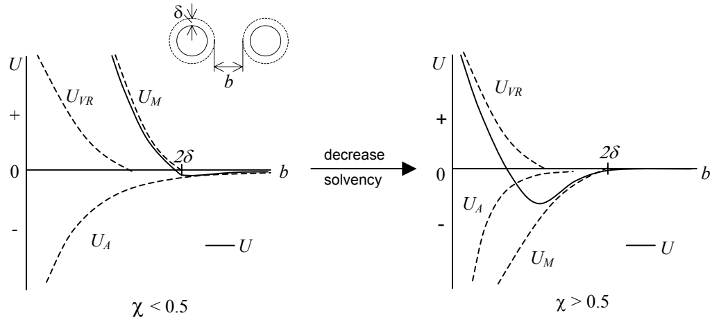
Figure 1.5. Sketch of interaction energies between two droplets stabilized by polymers.
