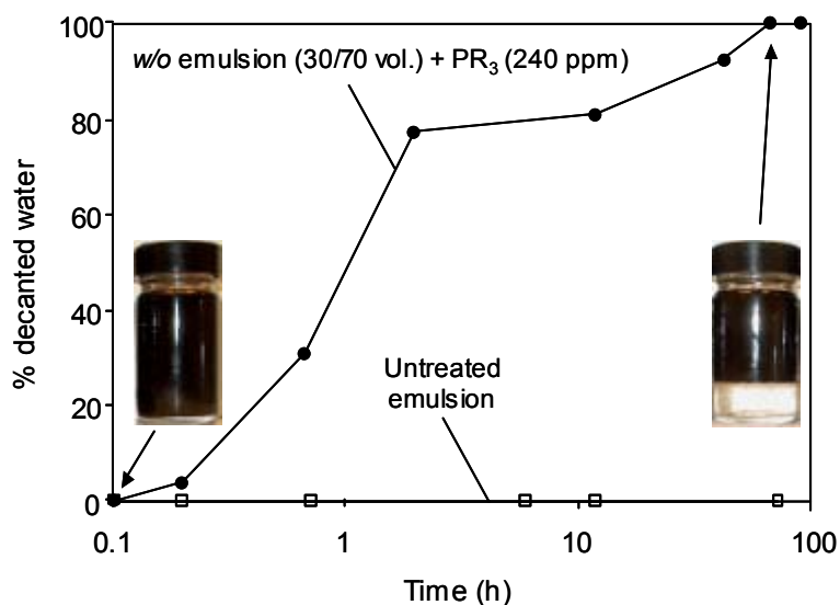
Figure 4.11. Bottle test results for an untreated emulsions (squares) and for an emulsion treated with the phenolic resin PR 3 (filled circles). The inserted pictures show the appearance of the bottles at the beginning and end of the test when the resin PR 3 was used.
