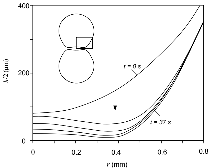
Figure 1.6. Transient behavior of a thin liquid film. The arrow indicates the direction in which the interface is displaced. The inserted drawing illustrates the section of the interface that is shown. The time lapse between initial and final positions is 37s. r_0 = 1 mm. h_0 = 160 nm. s = 0.5 . \sigma = 72 mN/m. Interaction forces have been neglected in these calculations.
