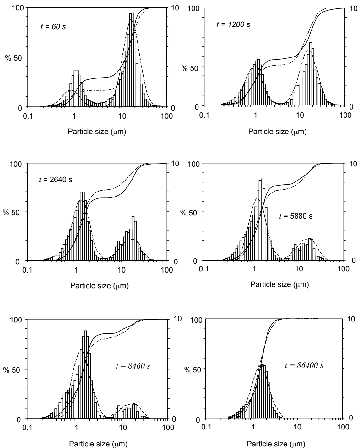
Figure 2.25. Case study 3: Transient behavior of the drop size distribution for the mixed emulsion. Solid bars and lines: Experimental data. Dashed lines: Results from numerical simulations.
