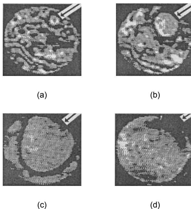
Figure 4.5. Stepwise drainage of an oil film stabilized by asphaltenes (7 vol.%) [22].
