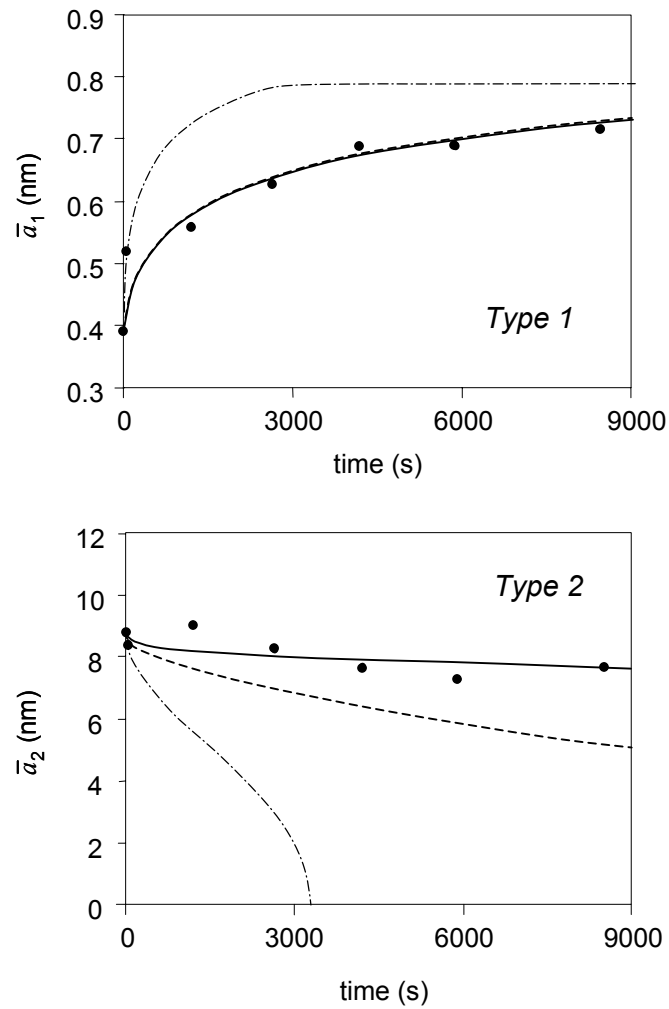
Figure 2.26. Case study 3: Transient behavior of the volume-weighted mean drop sizes of the two drop types present in the mixed emulsion. Dots: Experimental data. Solid lines: Numerical simulations with interface-controlled mass transfer model taking into account polydispersity in drop sizes. Dashed lines: Numerical simulations with interface-controlled mass transfer model neglecting polydispersity in drop sizes (Eq. [2.80]). Dash-and-dot lines: Numerical simulations with diffusion-controlled mass transfer model neglecting polydispersity in drop sizes (Eq. [2.82]).
