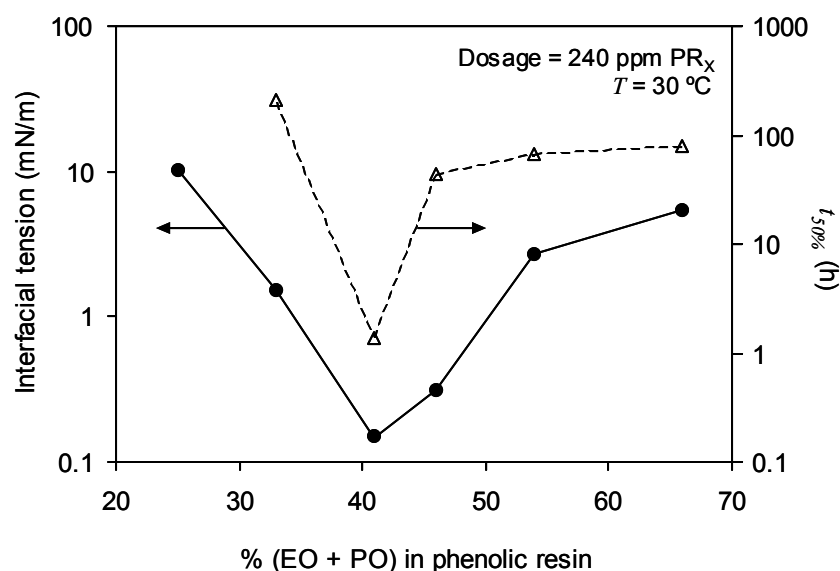
Figure 4.14. Effect of EO/PO content on the equilibrium interfacial tensions of emulsions treated with phenolic resins (filled circles). The times required in bottle tests to decant 50 % of the brine initially present in the emulsion are also plotted (triangles).
