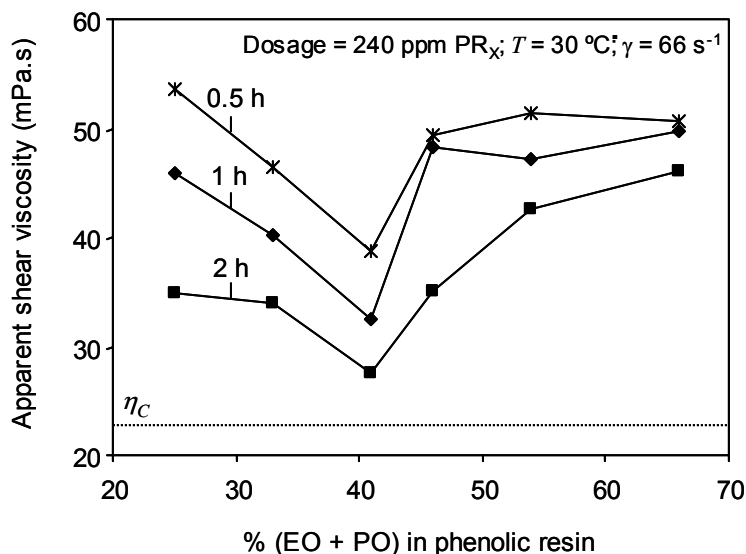
Figure 4.16. Effect of the EO/PO content of the phenolic resins on the transient behavior of the shear viscosity.
