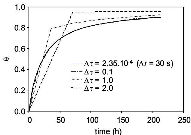
Figure 2.21. Case study 1: Effect of the selection of the time step \Delta\tau on the numerical response of the proposed algorithm for case study 1.
