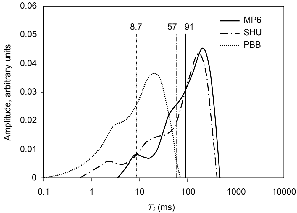
Figure 3.3. T_2 distributions of the oils used in this study.
