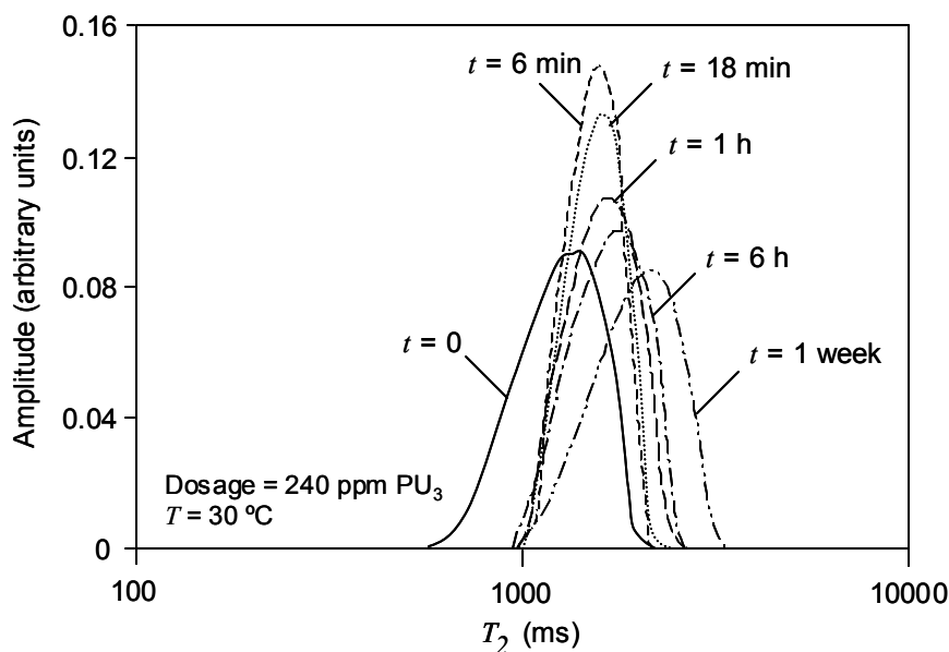
Figure 4.29. Evolution of the T_2 distribution of the water phase for an emulsion treated with 240 ppm of the cross-linked polyurethane PU_3 . The distribution of the oil phase has been omitted to simplify the interpretation of the plot.
