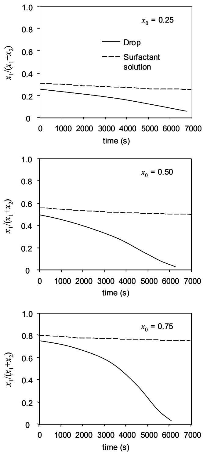
Figure 2.17. Predicted trends for the molar composition x_1/(x_1+x_2) of the oil drops and surfactant solutions for the solubilization of mixtures of n-decane (1) / n-undecane (2) in C_{12}E_8 (2.5 wt.%) at 30.9 °C.
