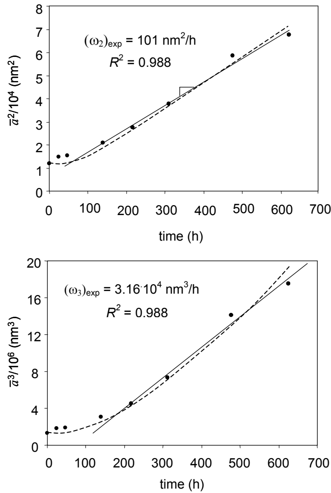
Figure 2.22. Case study 2: Experimental and numerical results for the transient behavior of the mean drop size. Top: plot of \bar{a}^2 vs. time. Bottom: plot of \bar{a}^3 vs. time. Black dots: experimental data. Solid lines: Linear fits at long ripening times. Dashed lines: Results from numerical simulations.
