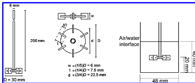
Figure 1. Sketch of the mixer and emulsion preparation.
