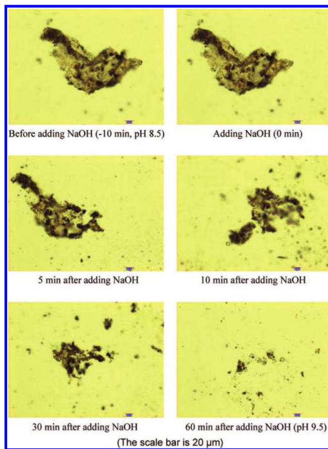
Figure 4. Clay solids skins with time when increasing pH from 8.5 to 9.5.
