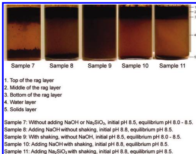
Figure 5. Pictures of 24 h emulsion after the top clean oil layer was removed.
