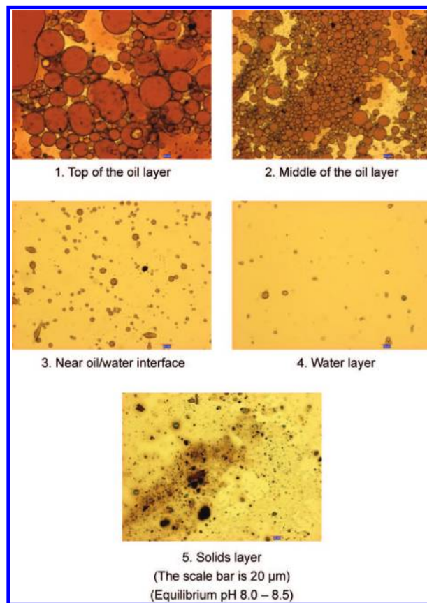
Figure 7. Emulsion (24 h) with shaking, without adding NaOH (sample 9).
