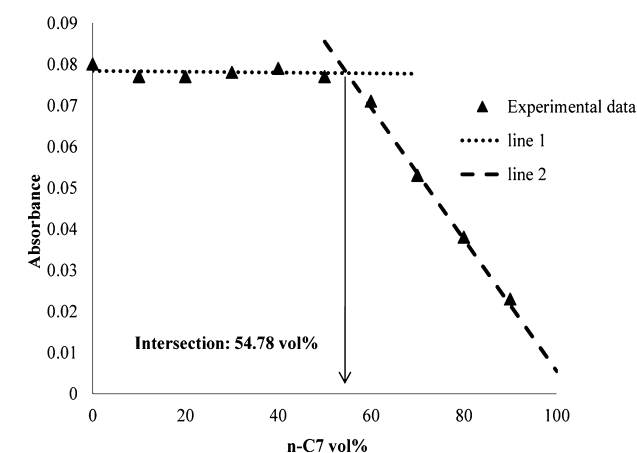
Figure 20. Precipitation onset measurement using an absorbance of UV-vis at 700 nm wavelength.
