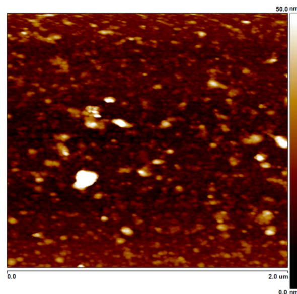
Figure 6. AFM image of the gold crystal surface after the QCM–D experiment using a n -C 5 asphaltene + toluene model oil system at 80 °C and at a 80 \mu\text{L}/\text{min} flow rate.
