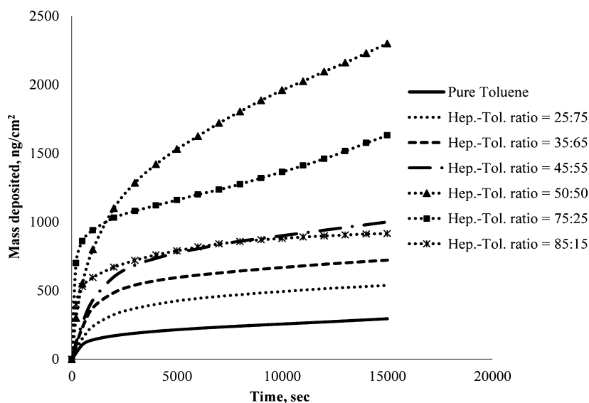
Figure 21. Effect of solvent on the amount of deposited mass from n -C 7 asphaltene + heptol systems onto a gold crystal surface versus time at 20 °C and at a 80 \mu L/min flow rate.
