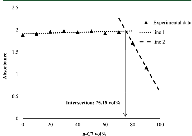
Figure 1. Precipitation onset measurement for a 1 h aged sample. The absorbance of UV-vis is 500 nm wavelength.
