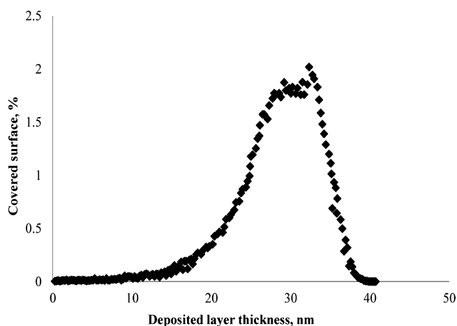
Figure 7. Thickness analysis of the AFM image shown in Figure 6
