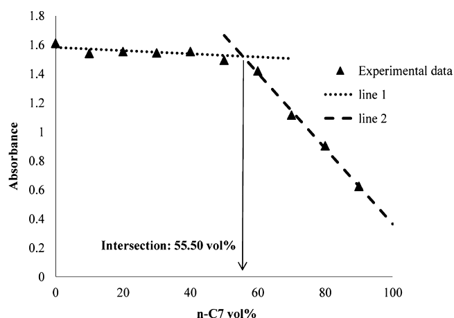
Figure 19. Precipitation onset measurement using an absorbance of UV-vis at 300 nm wavelength.
