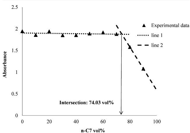
Figure 2. Precipitation onset measurement for a 24 h aged sample. The absorbance of UV-vis is 500 nm wavelength.
