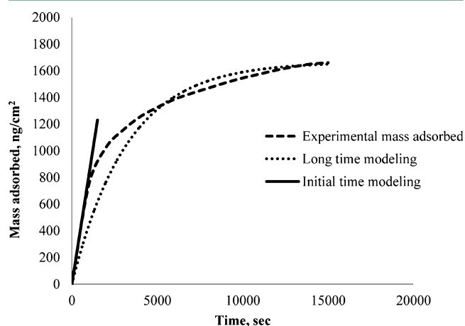
Figure 10. Experimental and modeling results for the amount of adsorbed mass from the n -C 5 asphaltene + toluene model oil onto a gold crystal surface versus time at 20 ^{\circ} C and at a 80 \mu L/min flow rate.
