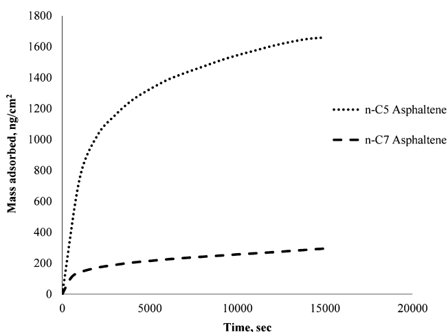
Figure 14. Amount of adsorbed mass from the model oil system onto a gold crystal surface versus time at 20 ^{\circ} C and at a 80 \mu L/min flow rate.
