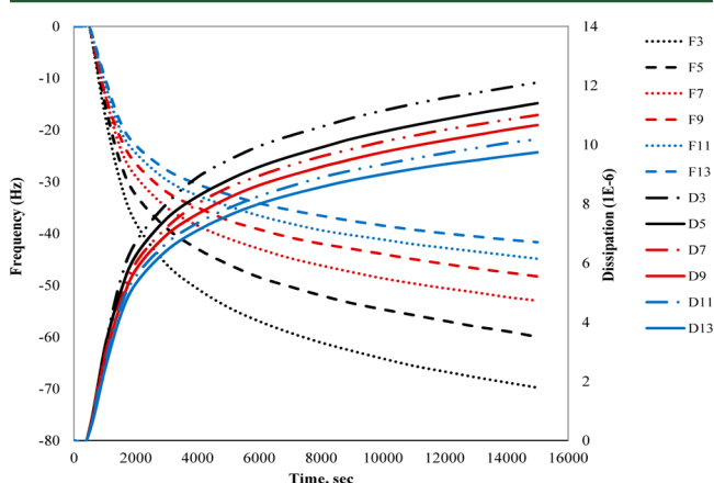
Figure 3. Frequency and dissipation changes versus time for the adsorption of n\text{-C}_5 asphaltene from the asphaltene + toluene system onto a gold quartz crystal surface.
