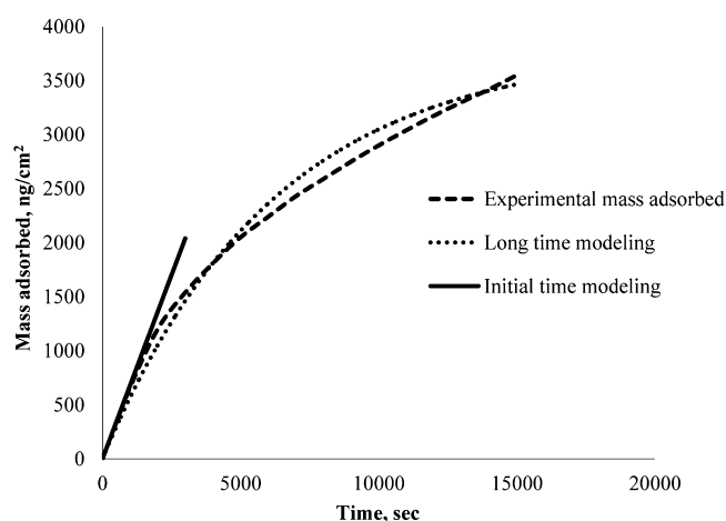
Figure 13. Experimental and modeling results for the amount of adsorbed mass from the n -C 5 asphaltene + toluene model oil onto a gold crystal surface versus time at 80 ^{\circ} C and at a 80 \mu L/min flow rate.
