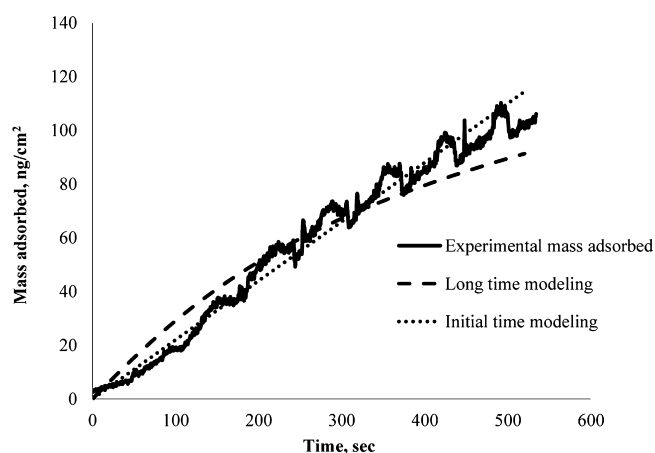
Figure 17. Comparison of experimental and modeling results for the amount of adsorbed mass from the n -C 7 asphaltene + toluene system onto a gold crystal surface at 20 °C during initial time. The flow rate is 80 µL/min.
