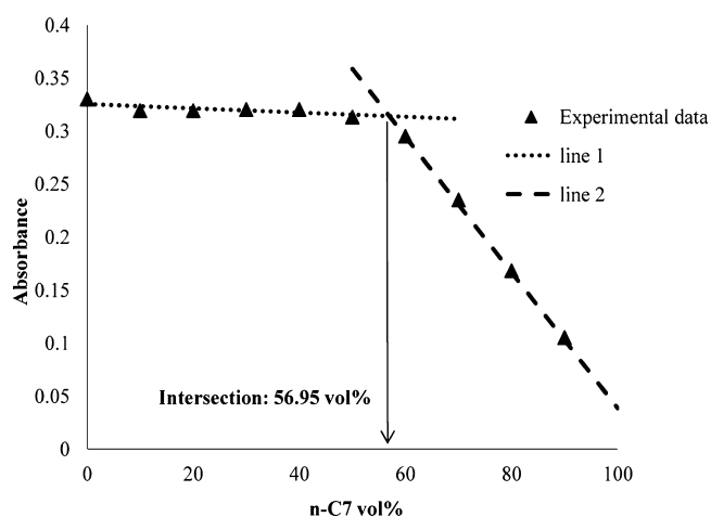
Figure 18. Precipitation onset measurement using an absorbance of UV-vis at 500 nm wavelength.
