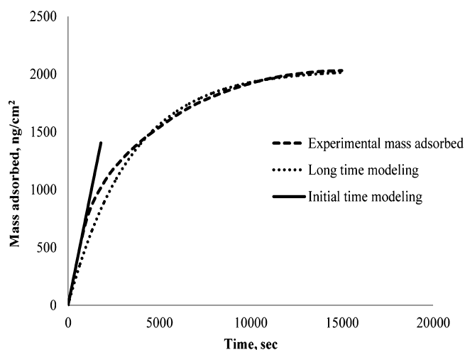
Figure 11. Experimental and modeling results for the amount of adsorbed mass from the n -C 5 asphaltene + toluene model oil onto a gold crystal surface versus time at 40 ^{\circ} C and at a 80 \mu L/min flow rate.
