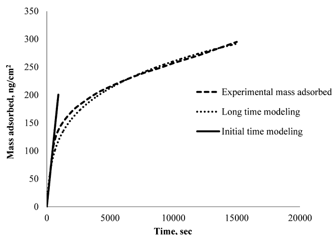
Figure 16. Experimental and modeling results for the amount of adsorbed mass from the n -C 7 asphaltene + toluene model oil onto a gold crystal surface versus time at 20 °C and at a 80 µL/min flow rate.
