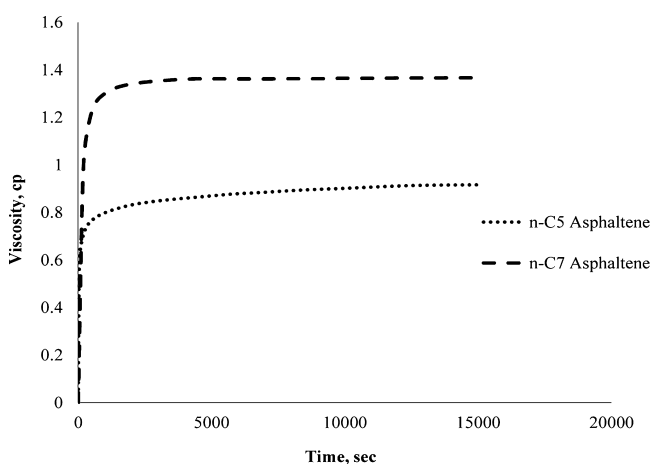
Figure 15. Viscosity of adsorbed mass from the model oil system onto a gold crystal surface versus time at 20 ^{\circ} C and at a 80 \mu L/min flow rate.
