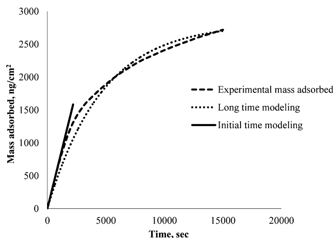
Figure 12. Experimental and modeling results for the amount of adsorbed mass from the n -C 5 asphaltene + toluene model oil onto a gold crystal surface versus time at 60 ^{\circ} C and at a 80 \mu L/min flow rate.
