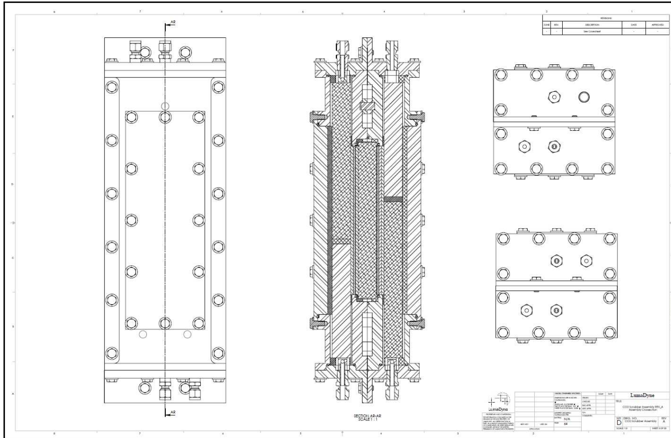
Figure 8.3 : An assembly cross-section view of the stainless steel prototype
