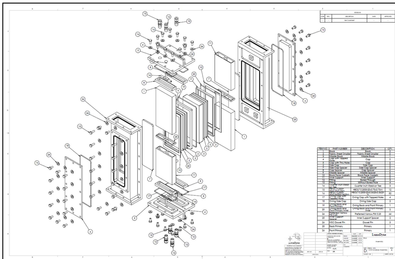
Figure 8.2 : An assembly view of the stainless steel prototype
