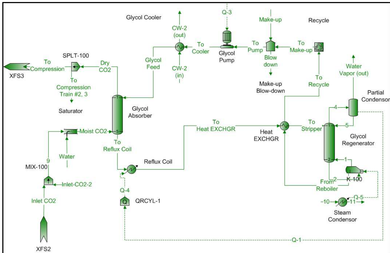
Figure 4.7 : Flowsheet for the glycol dehydration unit for conditioning CO 2 before transportation
