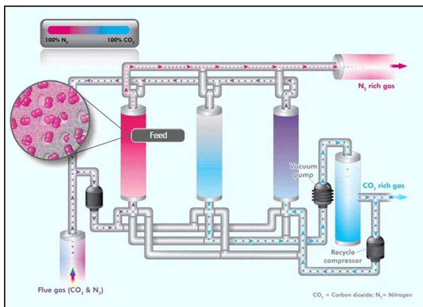
Figure 2.5 : Schematic representation of adsorption process for carbon dioxide ( \text{CO}_2 ) separation from flue gas [7]
