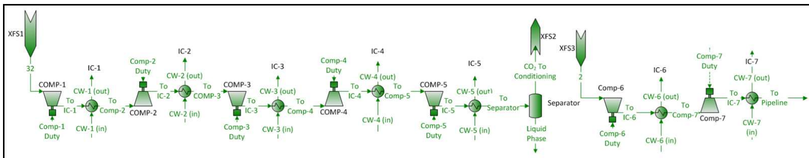
Figure 4.5 : Flowsheet for the compression of CO 2 separated with amine absorption trains using high pressure strippers
