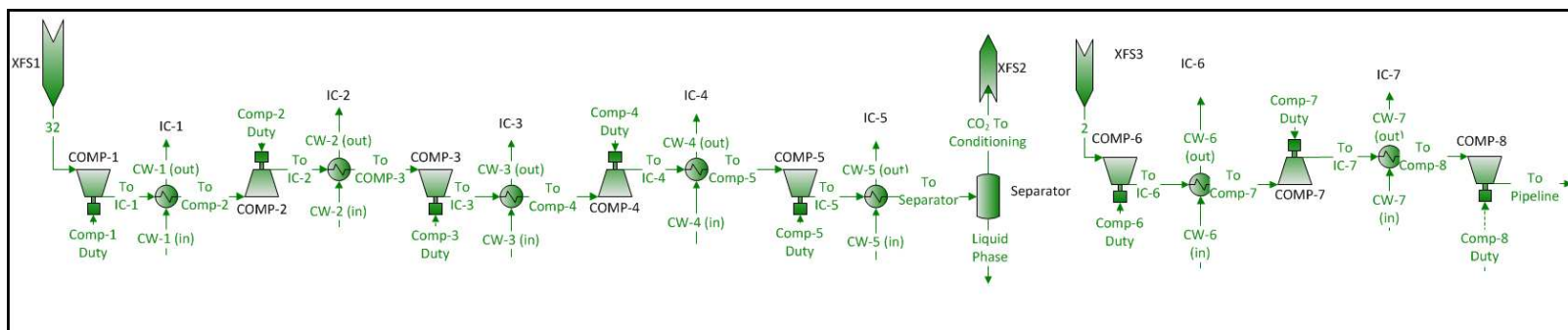
Figure 4.6 : Flowsheet for the compression of CO 2 separated with amine absorption trains using vacuum strippers
